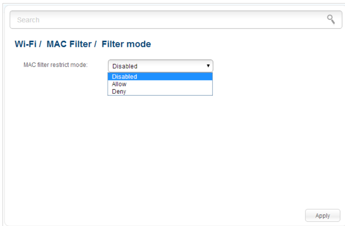
Figure 123. The page for configuring the MAC filter for the wireless network.
