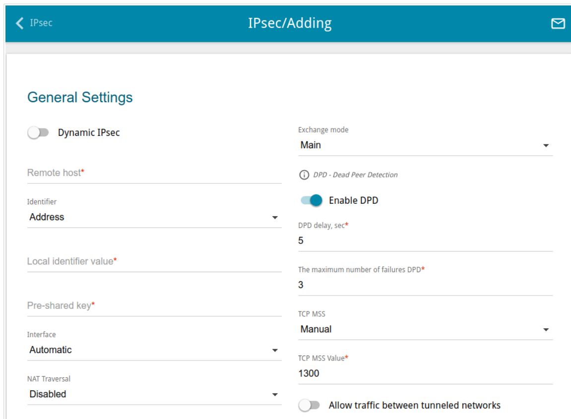
Figure 118. The page for adding an IPsec tunnel. The General Settings section.
