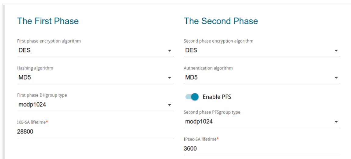
Figure 119. The page for adding an IPsec tunnel. The First Phase / The Second Phase sections.
