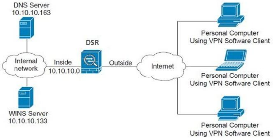
Figure 74: Example of three IPsec client connections to the internal network through the DSR IPsec gateway
