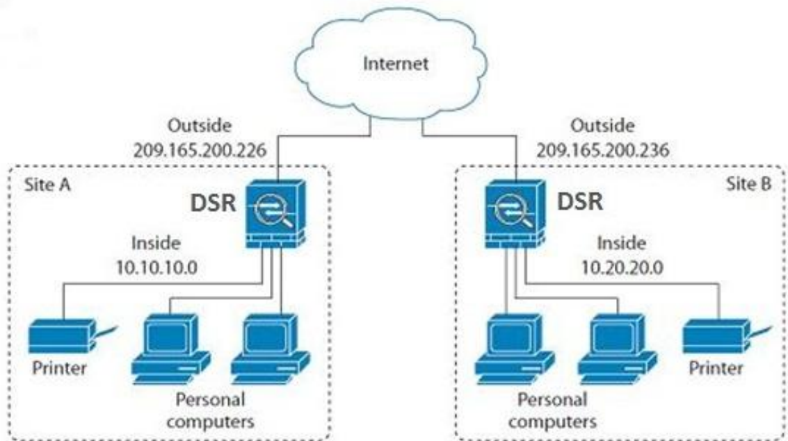
Figure 73: Example of Gateway-to-Gateway IPsec VPN tunnel using two DSR routers connected to the Internet
