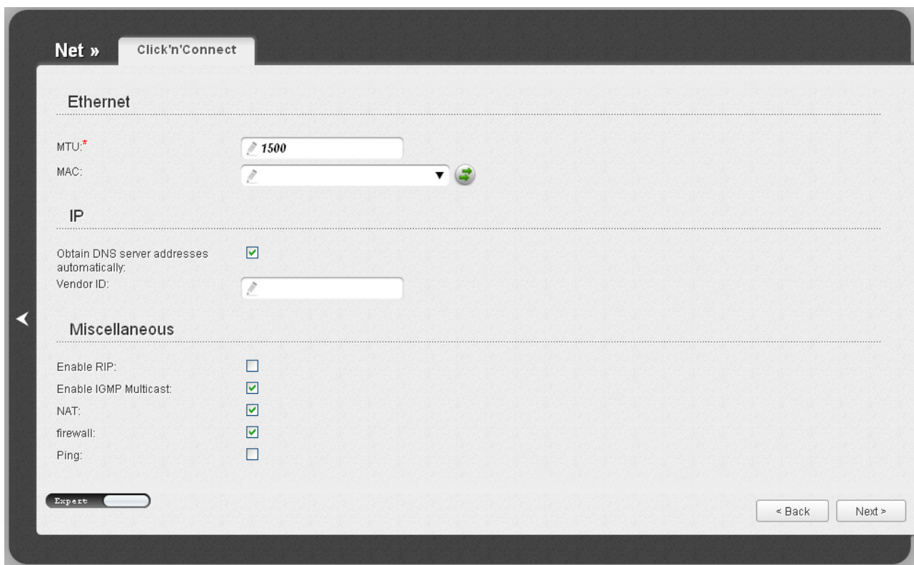
Figure 48. Configuring PPTP + Dynamic IP WAN connection. The expert settings mode. The IP and Miscellaneous sections.
