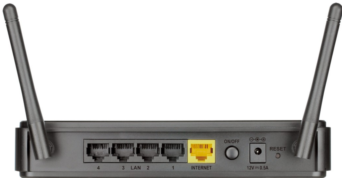
Figure 2. Back panel view.
