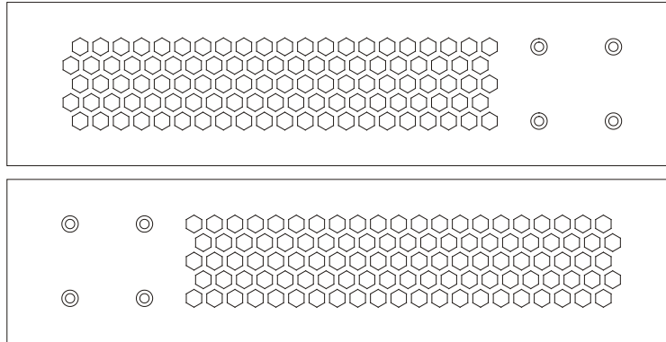
Figure 1- 16. Side panels of the DES-3200-10 and DES-3200-18
