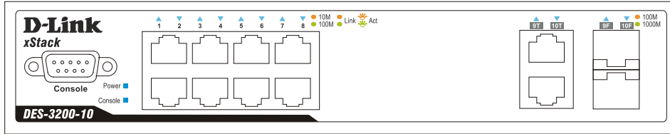
Figure 1- 6. Front Panel of the DES-3200-10
