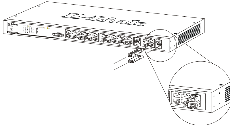
Figure 1- 19. Inserting the Mini-GBIC modules into the Switch
