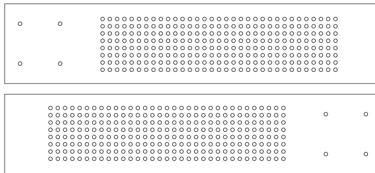
Figure 1- 17. Side panels of the DES-3200-26 and DES-3200-28
