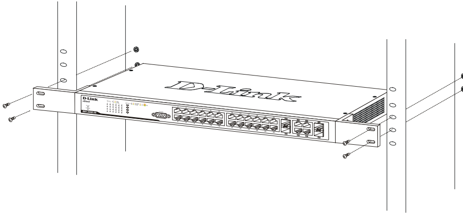
Figure 2 - 3. Installing Switch in a rack
