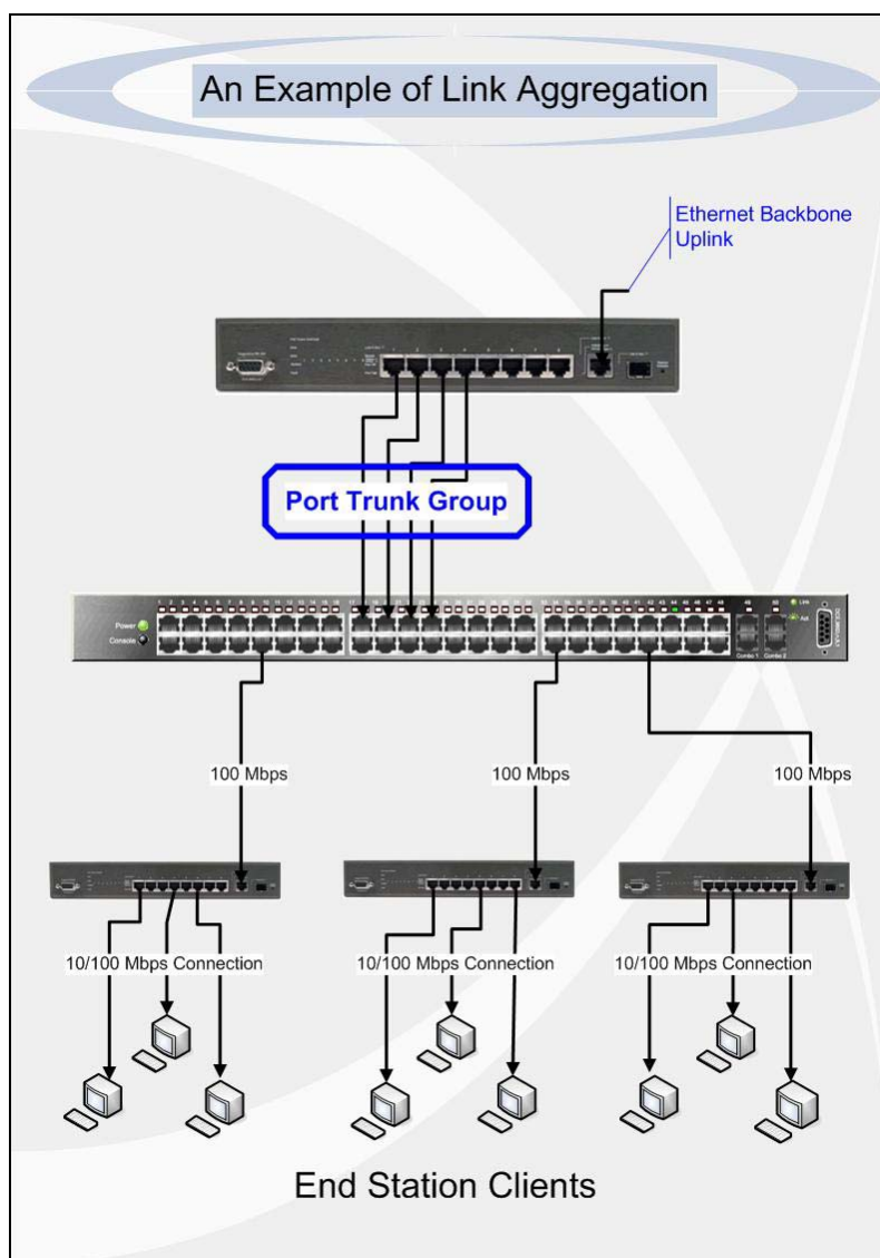
Figure 7- 16. Example of Port Trunk Group
