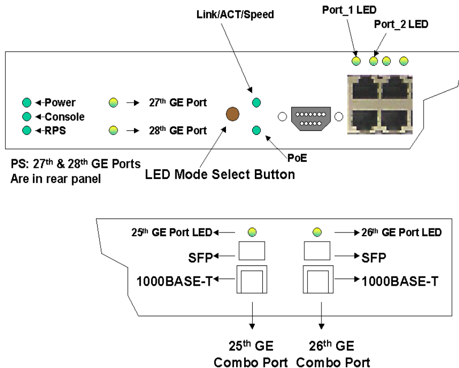
Figure 1- 4. Front Panel View of the DES-3828P
