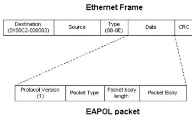
Figure 11- 3. The EAPOL Packet
