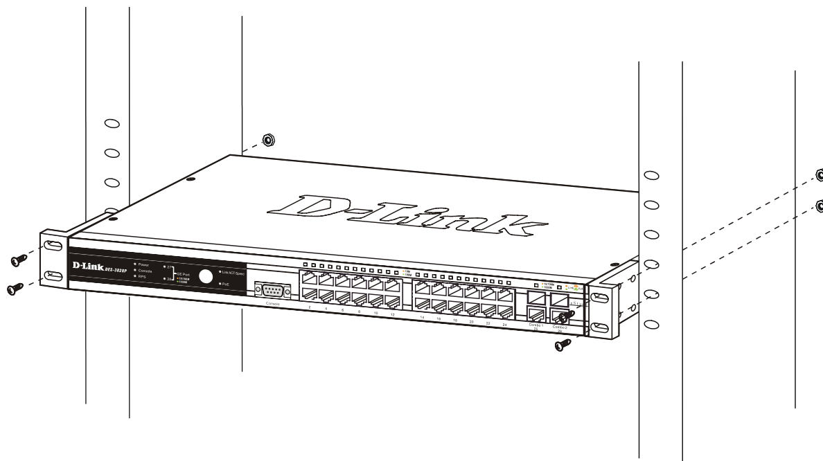
Figure 2 - 3. Installing Switch in a rack
