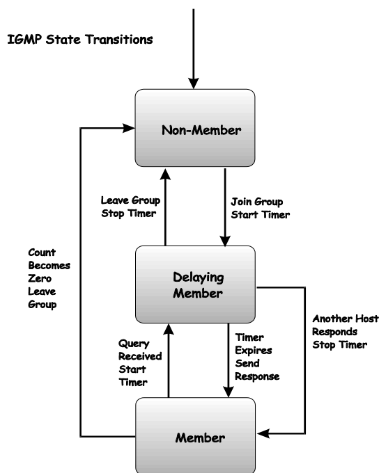
Figure 8- 53. IGMP State Transitions
