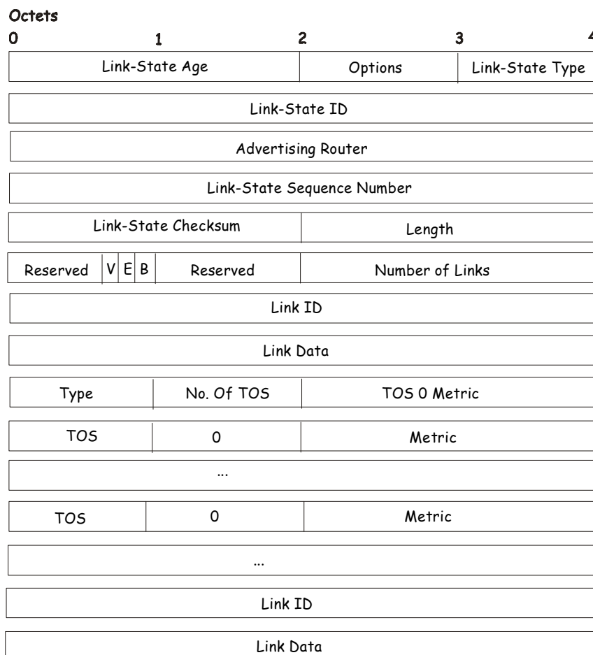
Figure 8- 24. Routers Links Advertisements
