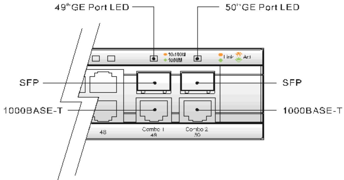
Figure 1- 6. LED Indicators for the DES-3852
