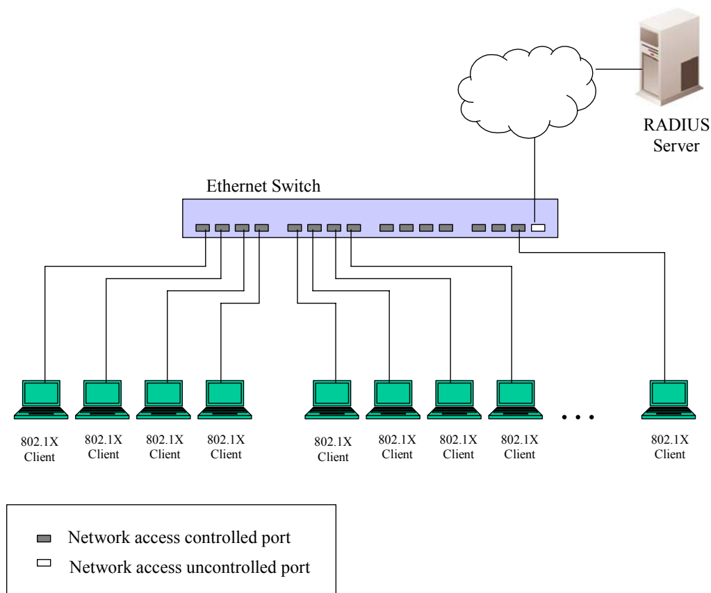
Figure 11- 9. Example of Typical Port-Based Configuration
