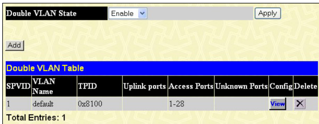
Figure 7- 13 Double VLAN Table (enabled)
