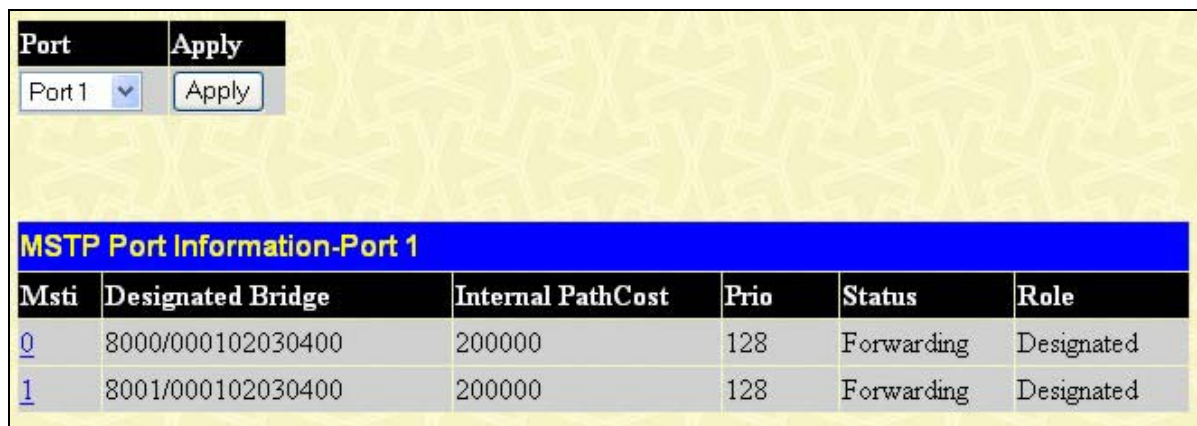
Figure 7- 32. MSTP Port Information window
