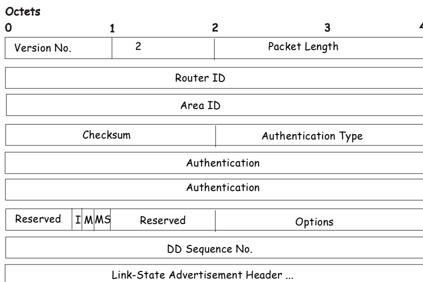
Figure 8- 19. Database Description Packet
