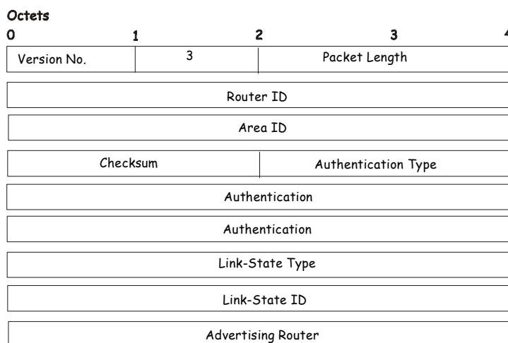
Figure 8- 20. Link-State Request Packet
