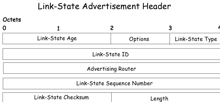
Figure 8- 23. Link State Advertisement Header
