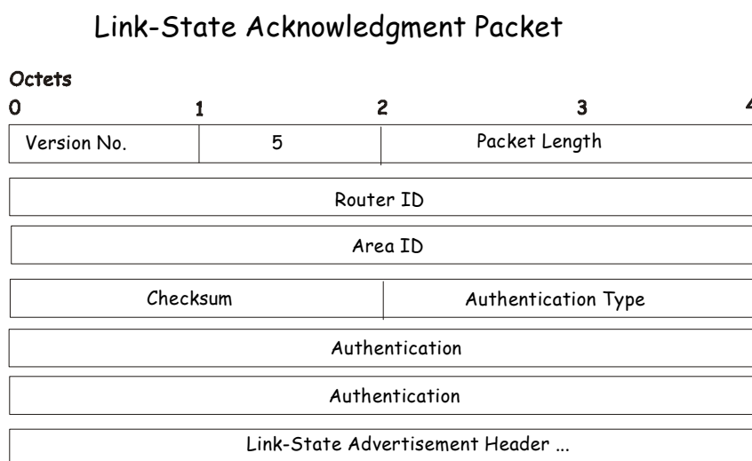
Figure 8- 22. Link State Acknowledge Packet
