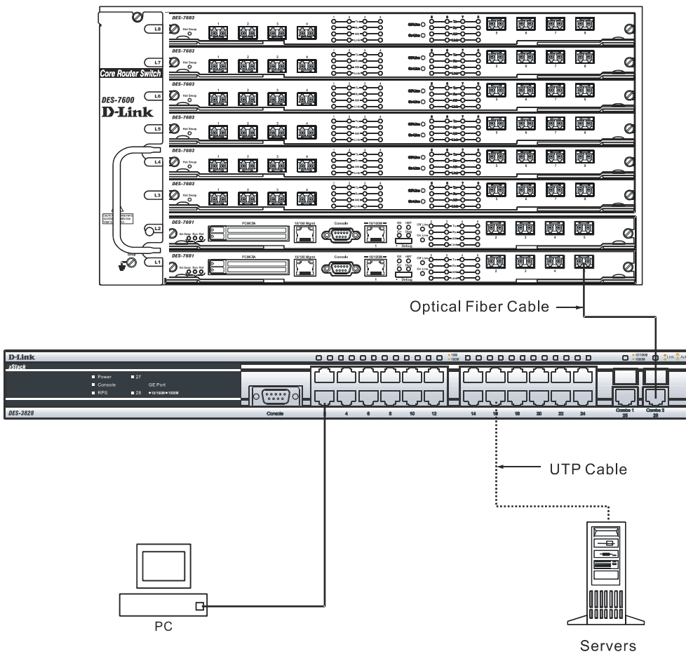
Figure 3- 3. Uplink Connection to a server, PC or switch stack.
