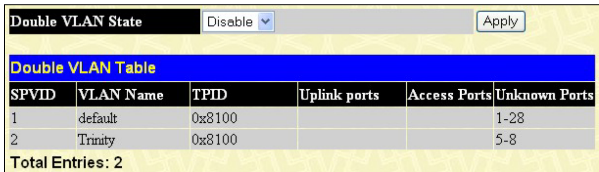
Figure 7- 12. Double VLAN Table (disabled)
