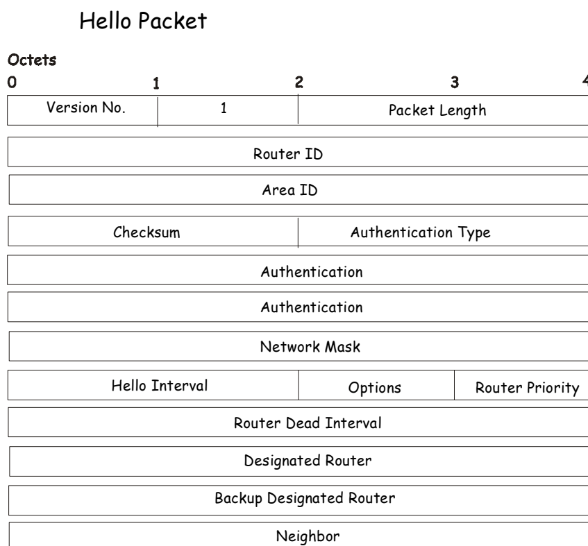
Figure 8- 18. Hello Packet
