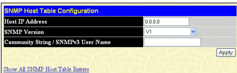
Figure 6- 32. SNMP Host Table Configuration window
