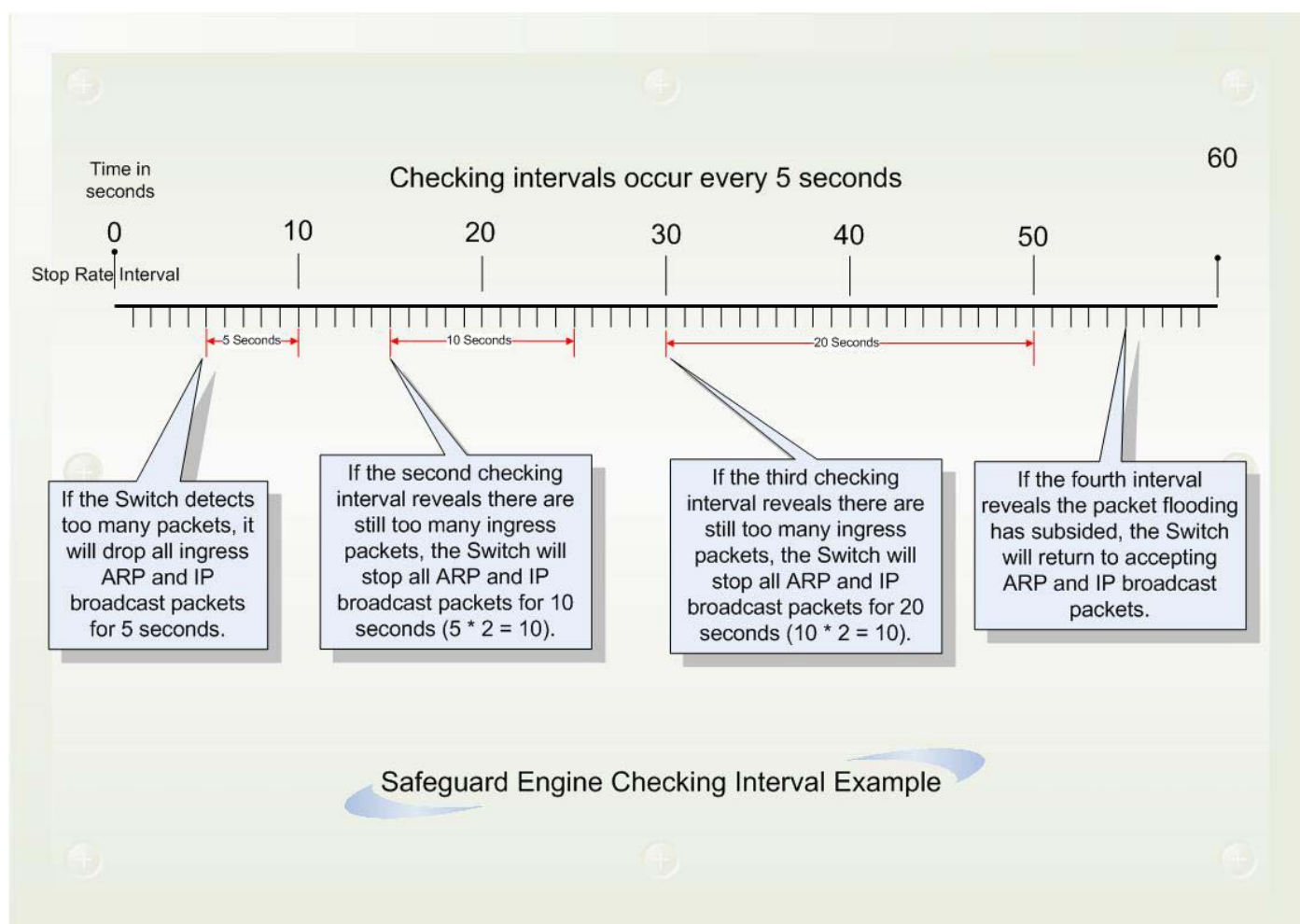
Figure 11- 47. Safeguard Engine example
