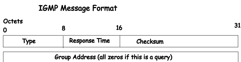
Figure 8- 52. IGMP Message Format
