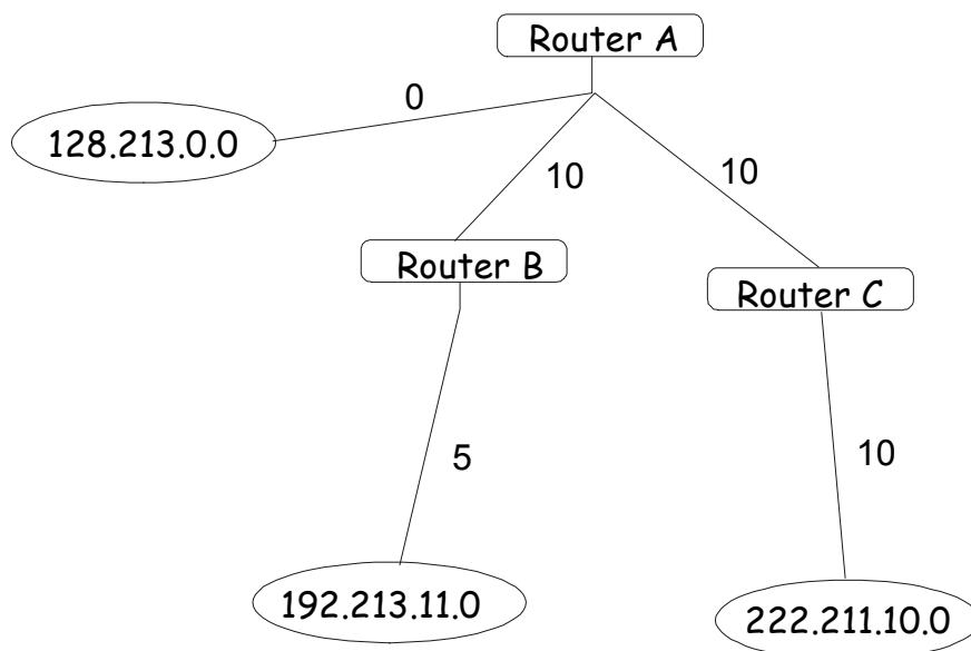
Figure 8- 16. Constructing a Shortest Path Tree - Completed
