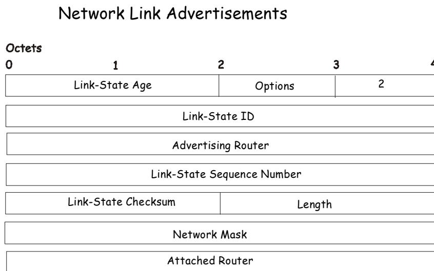
Figure 8- 25. Network Link Advertisements
