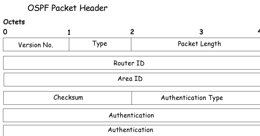
Figure 8- 17. OSPF Packet Header Format
