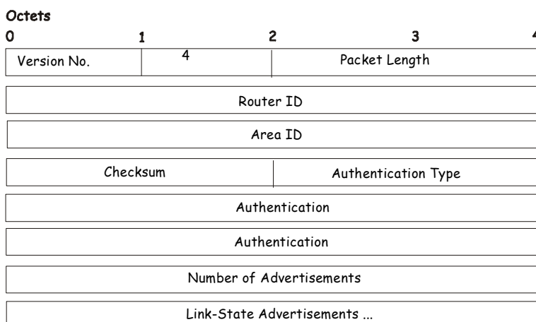
Figure 8- 21. Link-State Update Packet
