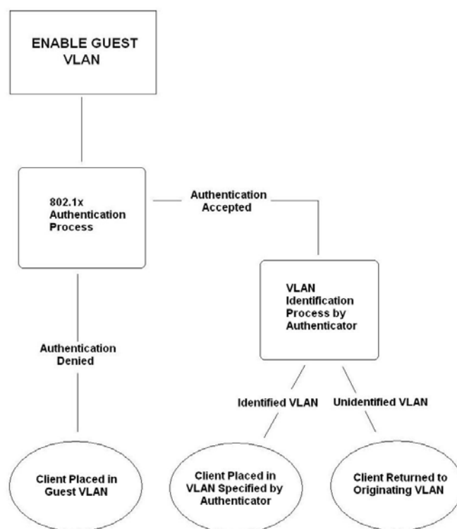
Figure 7- 5. Guest VLAN Authentication Process
