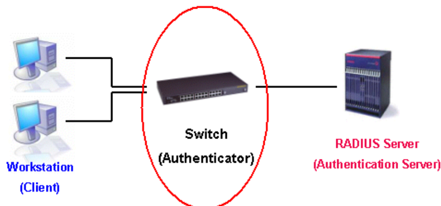
Figure 11- 6. The Authenticator
