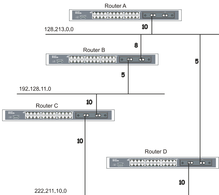
Figure 8- 14. Constructing a Shortest Path Tree
