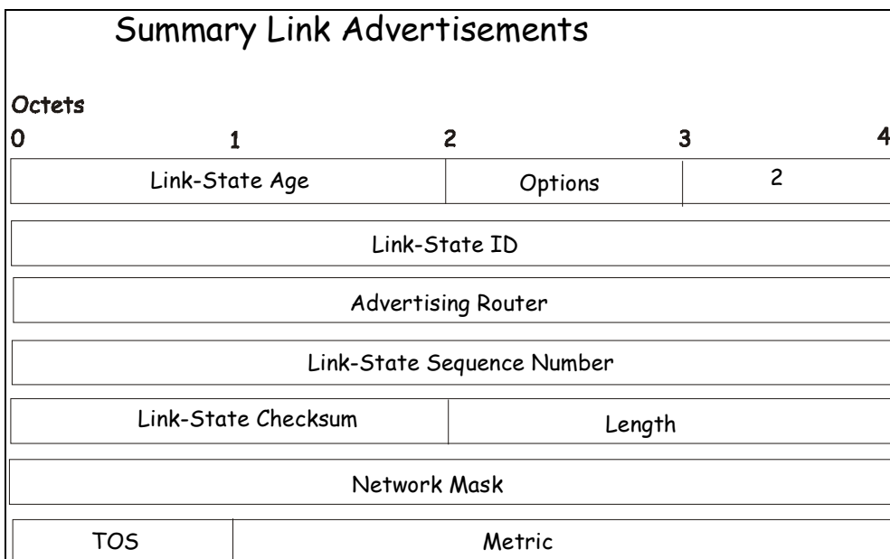
Figure 5-40 Summary Link Advertisements
