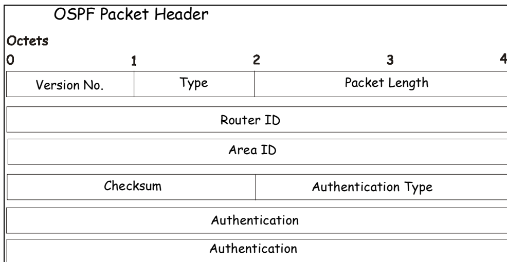
Figure 5-31 OSPF Packet Header Format
