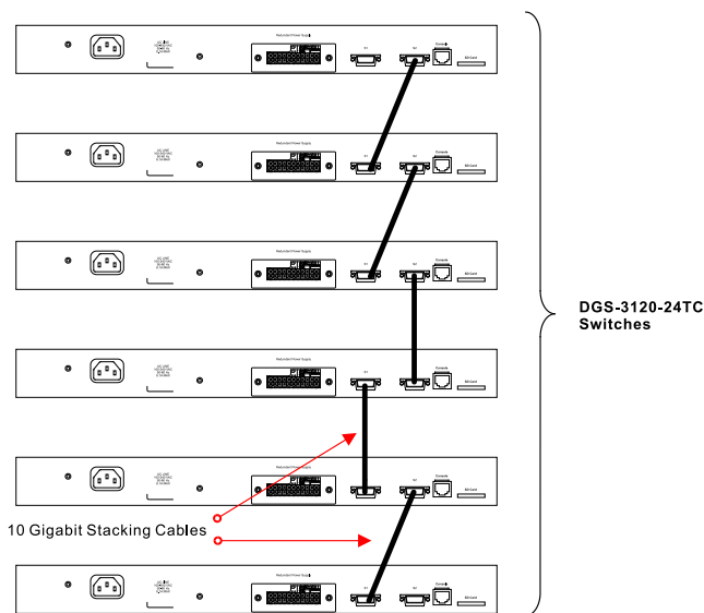
Figure 2-35 Switches stacked in a Duplex Chain
