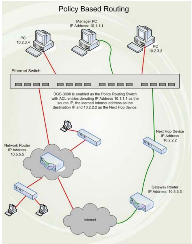
Figure 5-13 Policy Base Routing Example window
