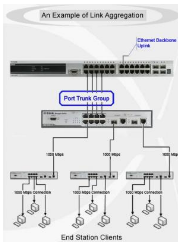
4-40 Example of Port Trunk Group
