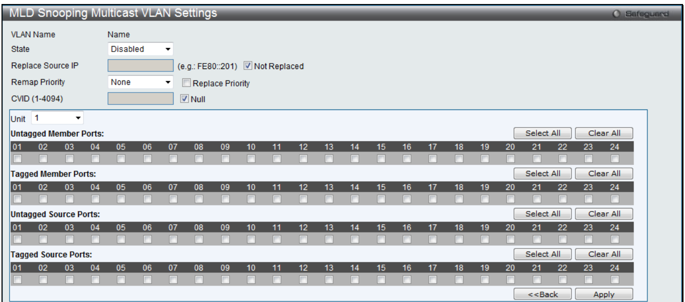
Figure 4-96 MLD Snooping Multicast VLAN Settings – Edit window
