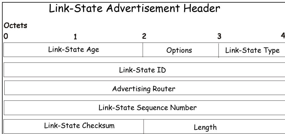
Figure 5-37 Link State Advertisement Header
