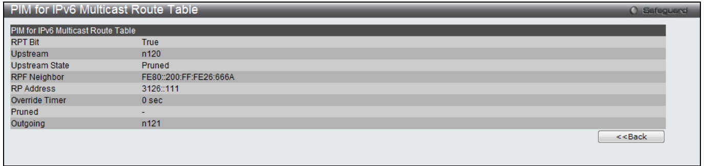
Figure 5-128 PIM for IPv6 Multicast Route Table - View Detail window
