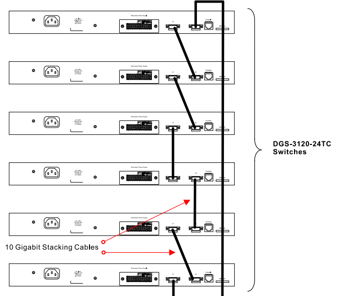
Figure 2-36 Switches stacked in a Duplex Ring
