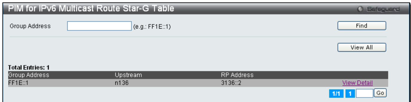
Figure 5-130 PIM for IPv6 Multicast Route Star-G Table window
