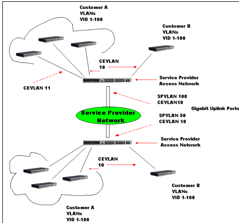
Figure 4-31 QinQ example window
