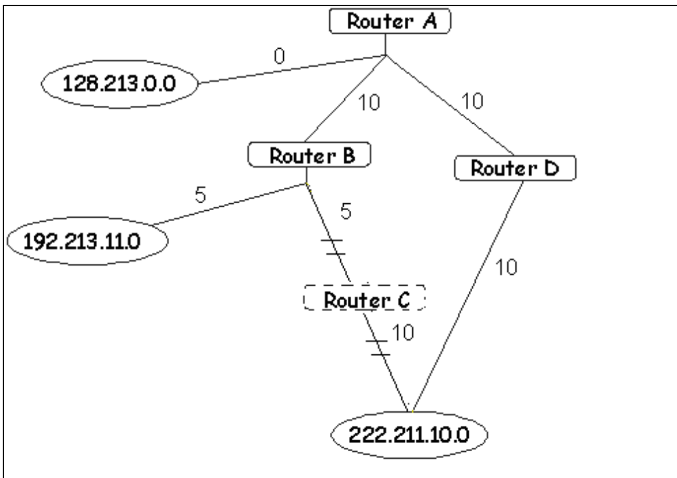
Figure 5-29 Constructing a Shortest Path Tree
