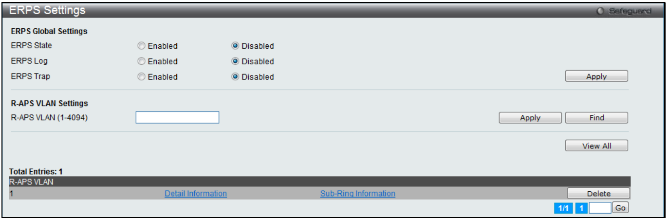
Figure 4-107 ERPS Settings Window
