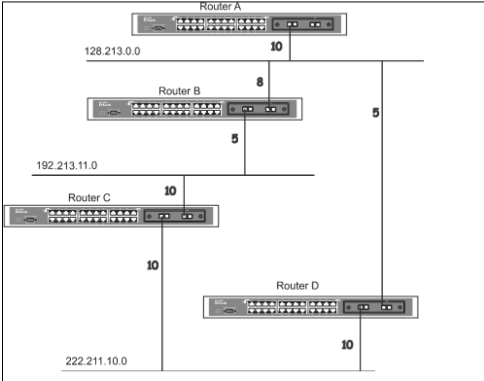
Figure 5-28 Constructing a Shortest Path Tree
