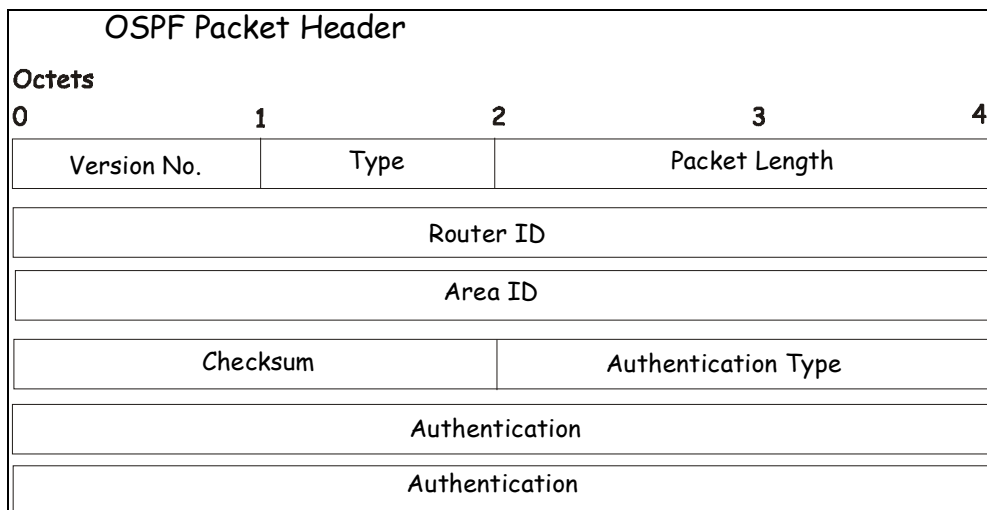
Figure 5-31 OSPF Packet Header Format
