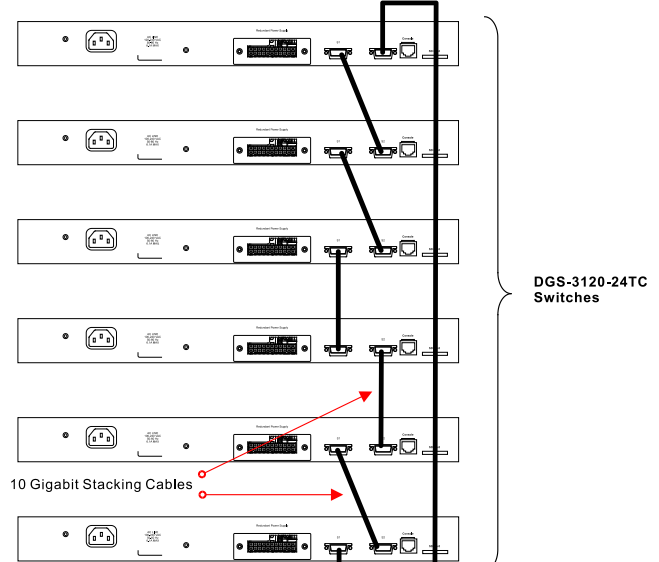
Figure 2-36 Switches stacked in a Duplex Ring
