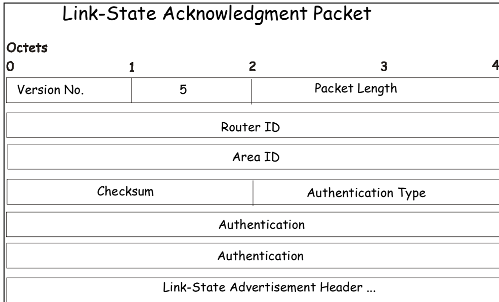
Figure 5-36 Link State Acknowledge Packet
