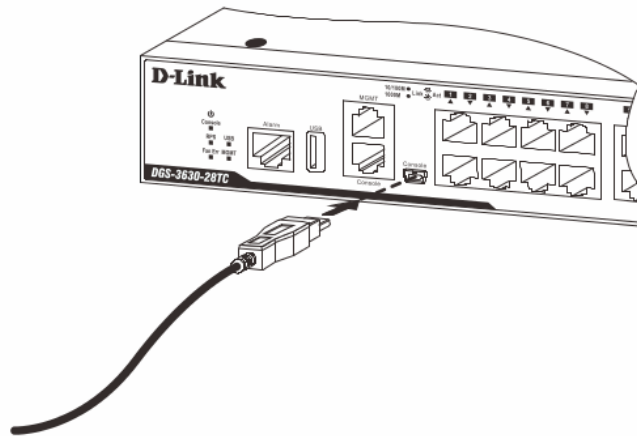
Figure 7 — Connect mini-USB Console Port
