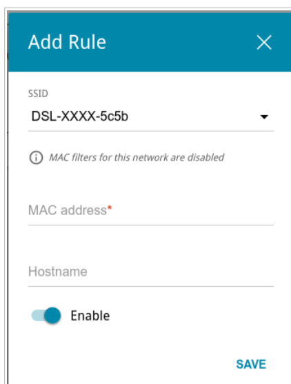
Figure 92. The window for adding a rule for the MAC filter.
