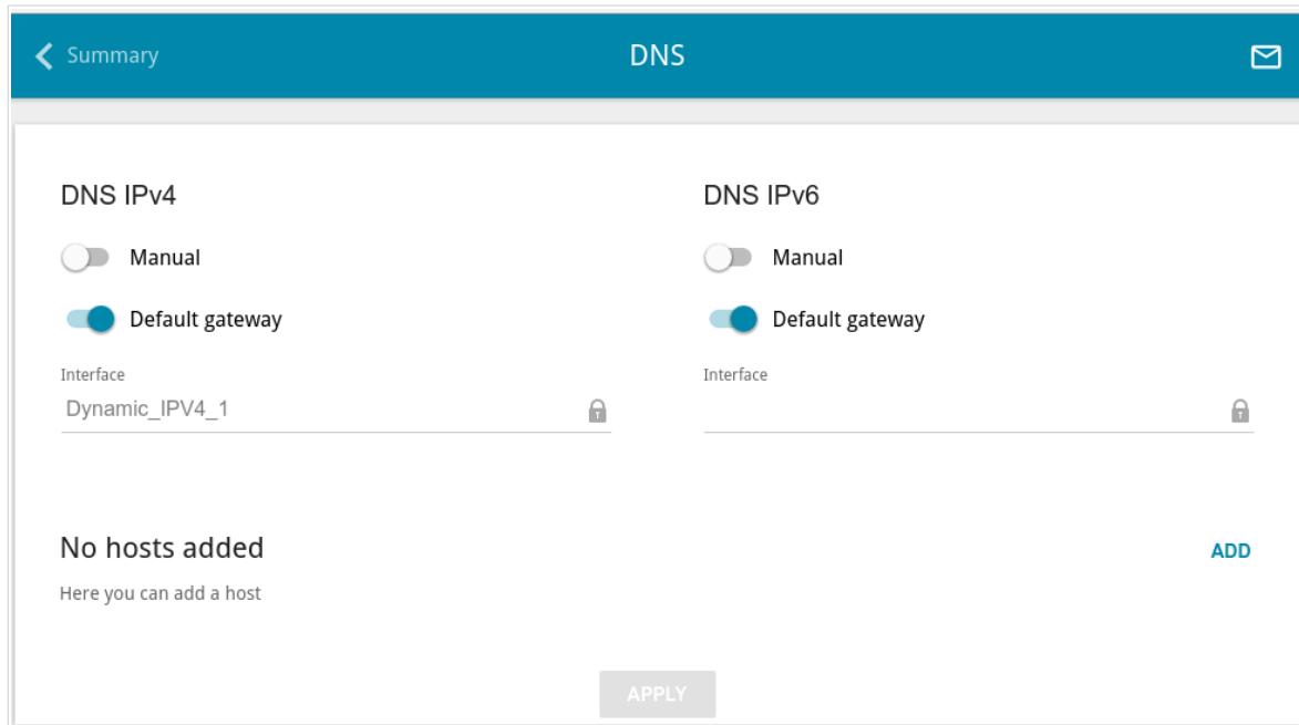
Figure 96. The Advanced / DNS page.
