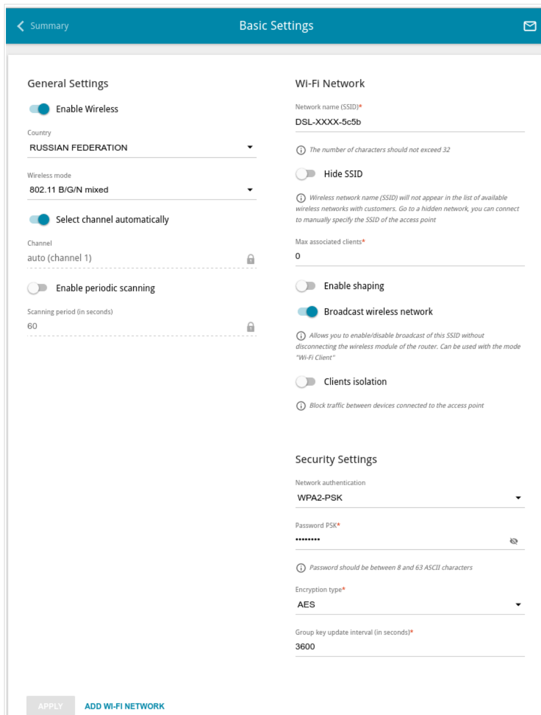
Figure 80. Basic settings of the wireless LAN.
