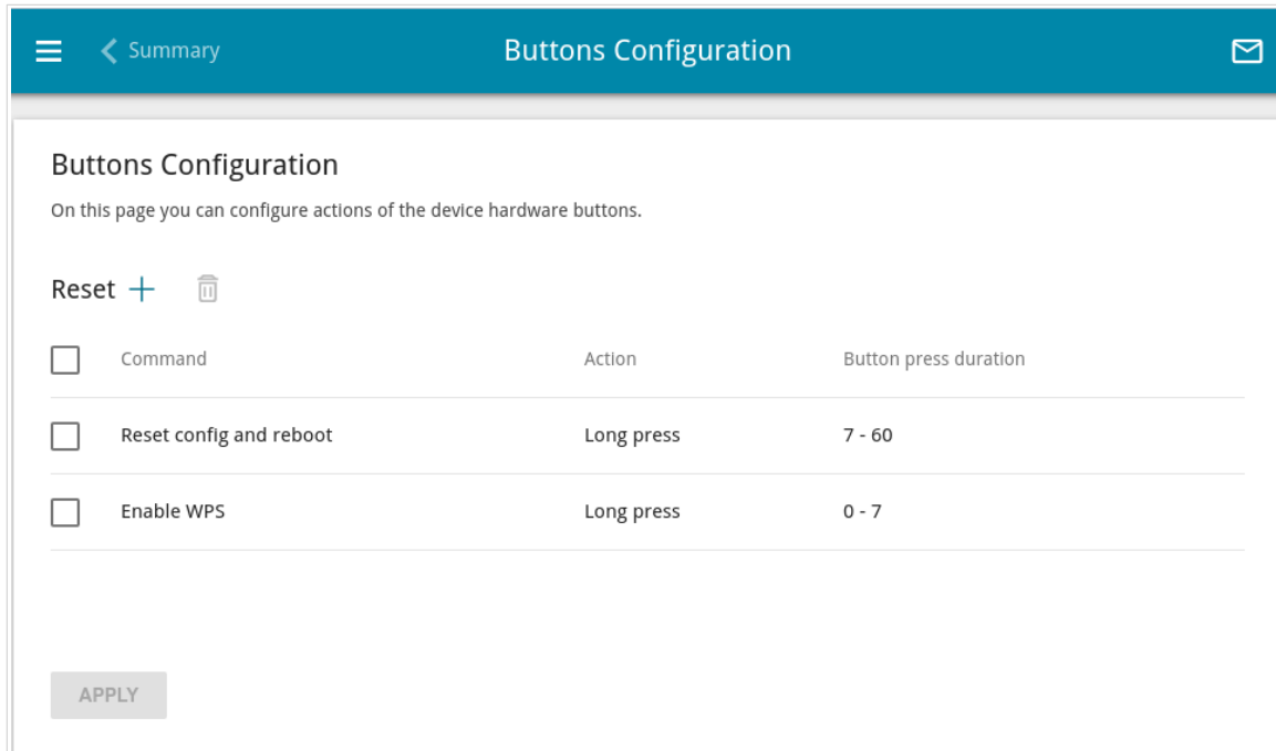
Figure 139. The System / Buttons Configuration page.
