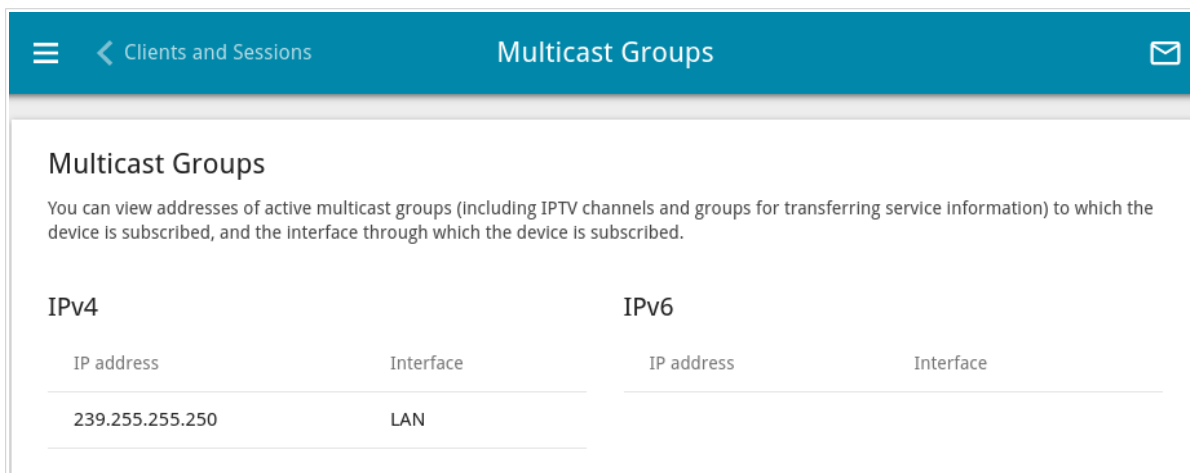
Figure 60. The Statistics / Multicast Groups page.
