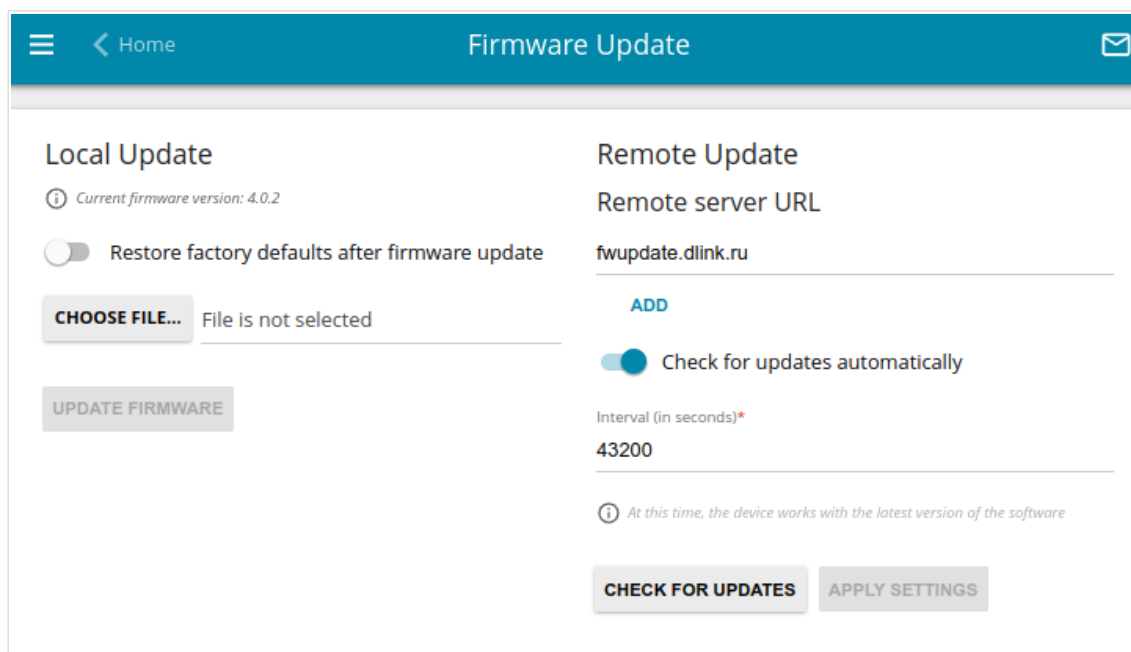
Figure 141. The System / Firmware Update page.
