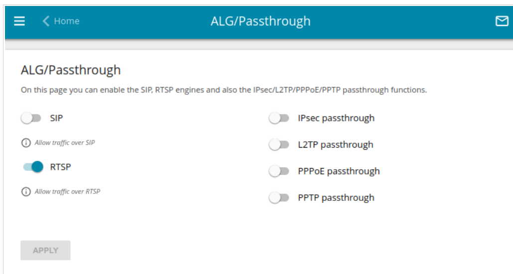
Figure 126. The Advanced / ALG/Passthrough page.
