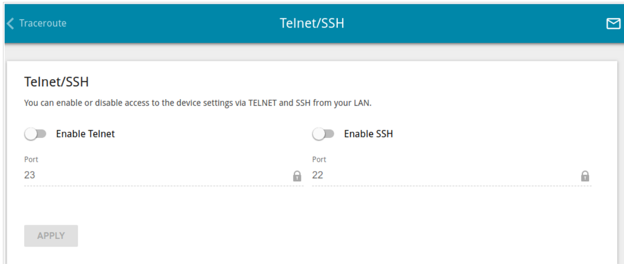
Figure 151. The System / Telnet/SSH page.
