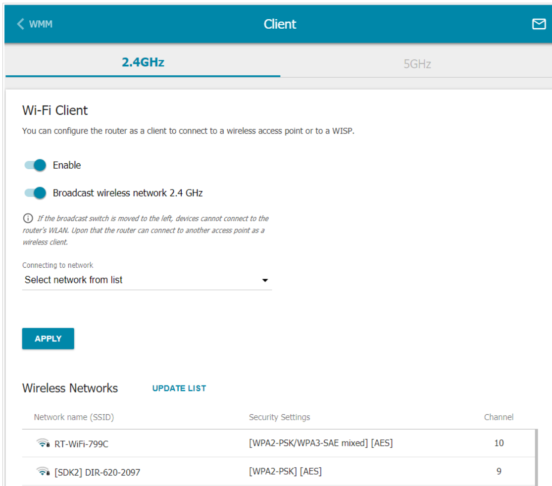
Figure 103. The page for configuring the client mode.
