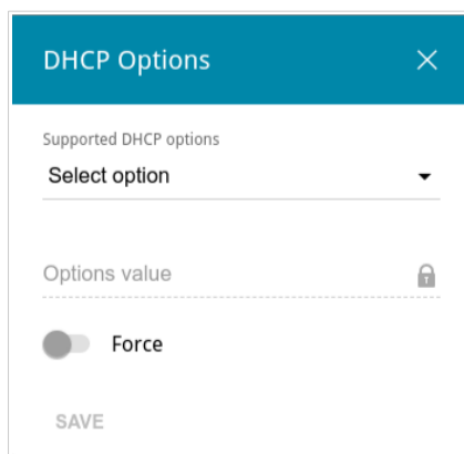
Figure 84. Configuring the local interface. The IPv4 tab. The window for configuring a DHCP option.
