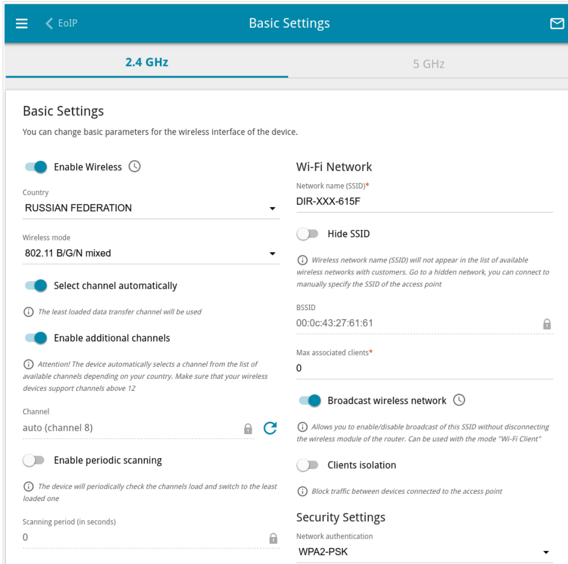
Figure 93. Basic settings of the wireless LAN in the 2.4GHz band.
