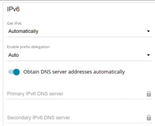
Figure 80. The page for creating a new PPPoE Pv6 connection. The IPv6 section.
