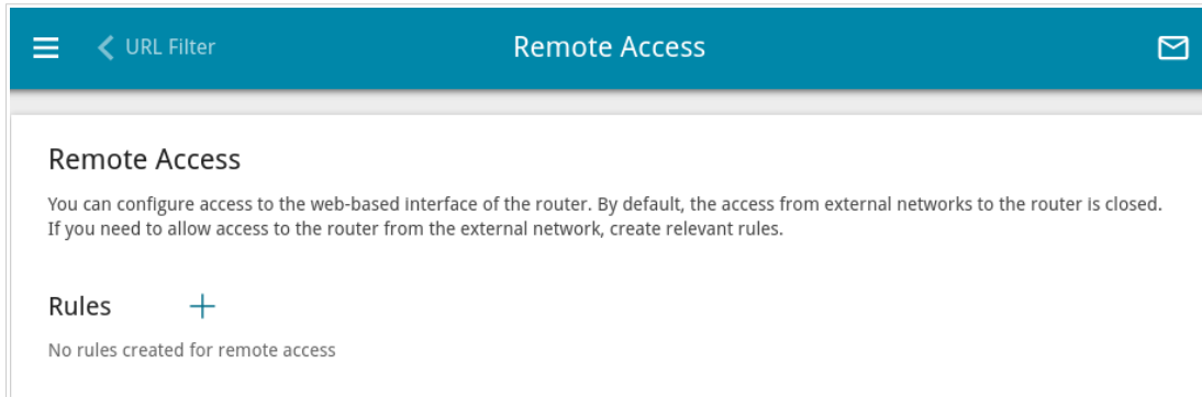
Figure 136. The Firewall / Remote Access page.
