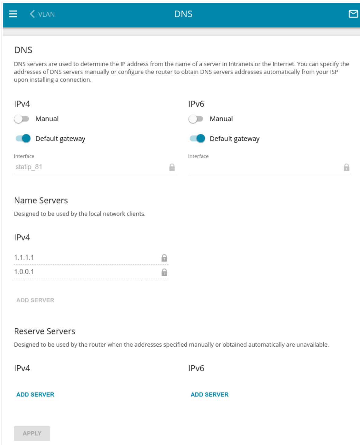
Figure 113. The Advanced / DNS page.
