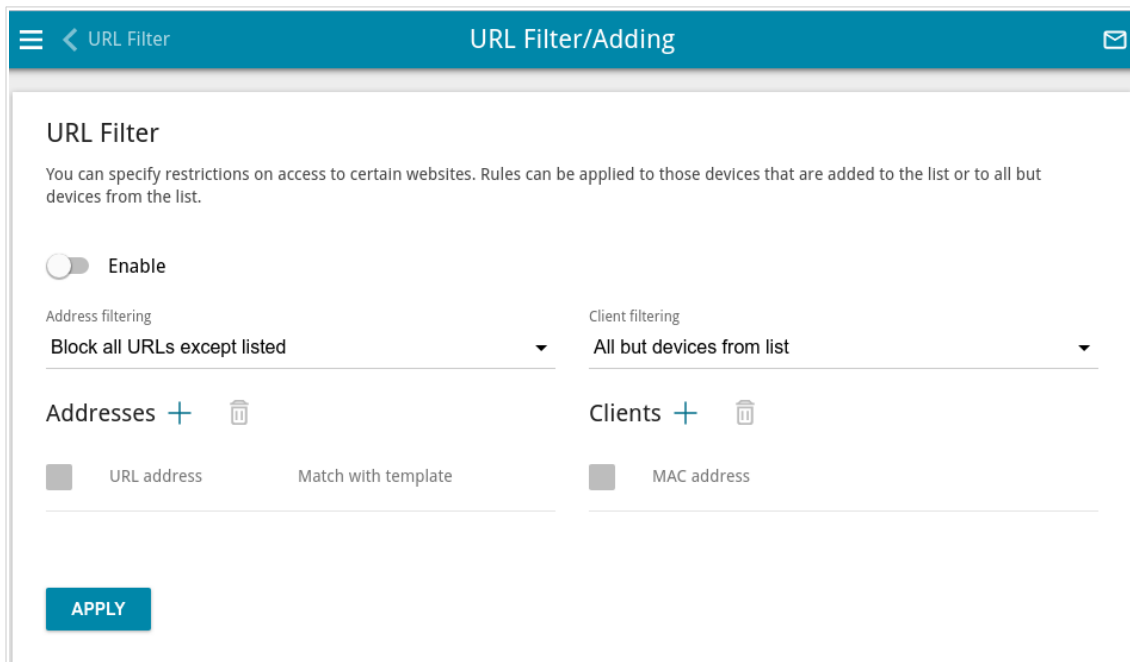
Figure 135. The page for adding a rule for URL filter.
