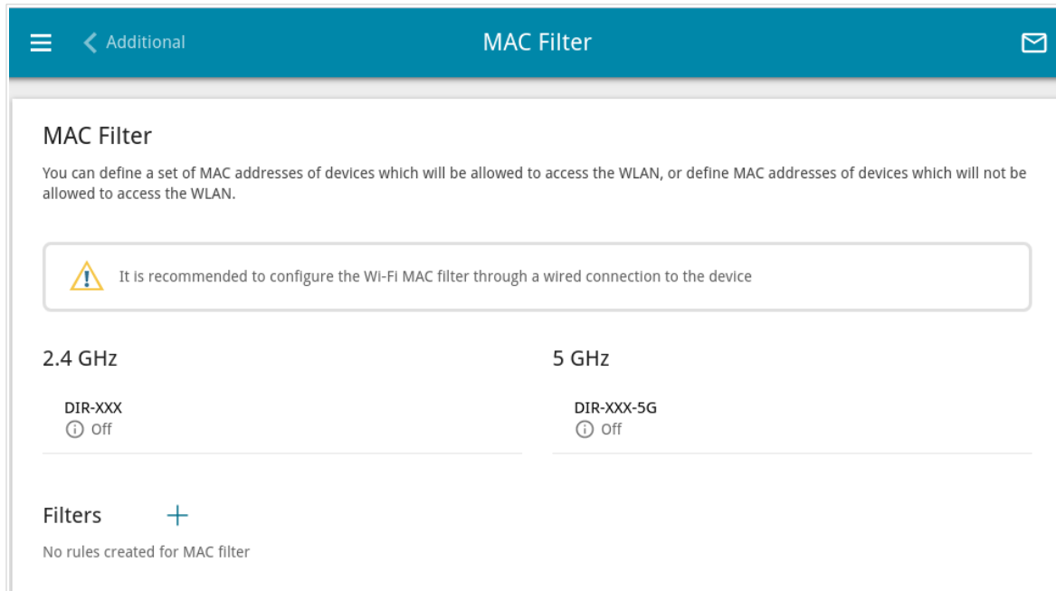
Figure 105. The page for configuring the MAC filter for the wireless network.
