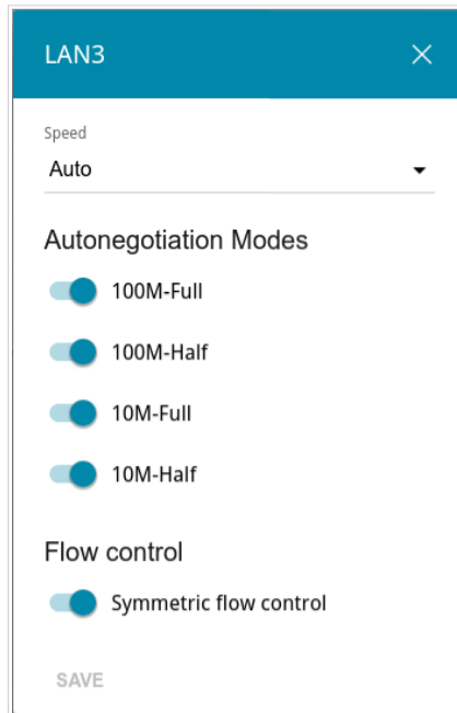
Figure 117. The window for changing the settings of the router's port.
