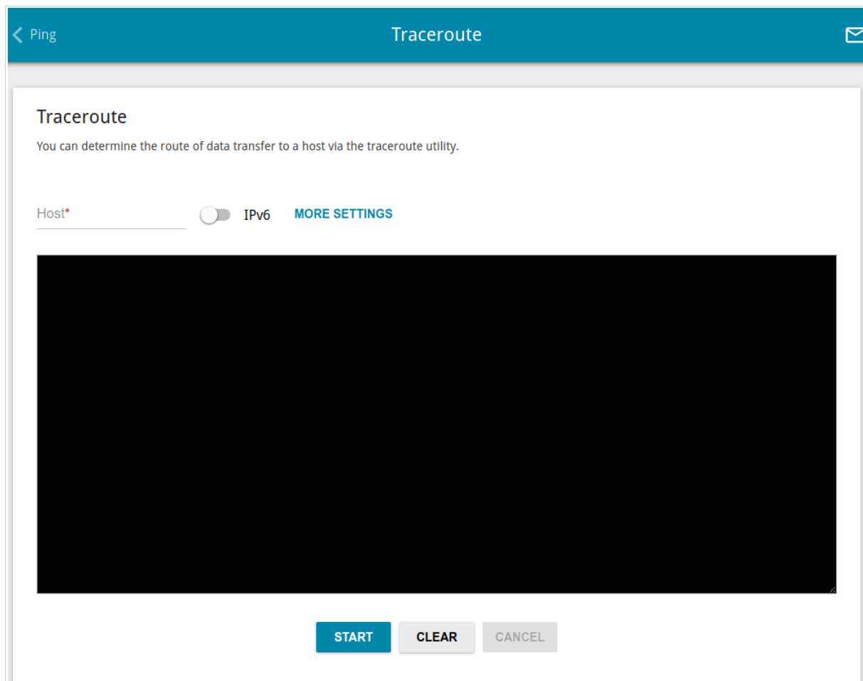
Figure 149. The System / Traceroute page.
