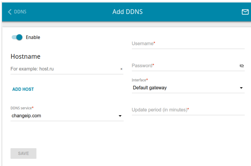
Figure 115. The page for adding a DDNS service.
