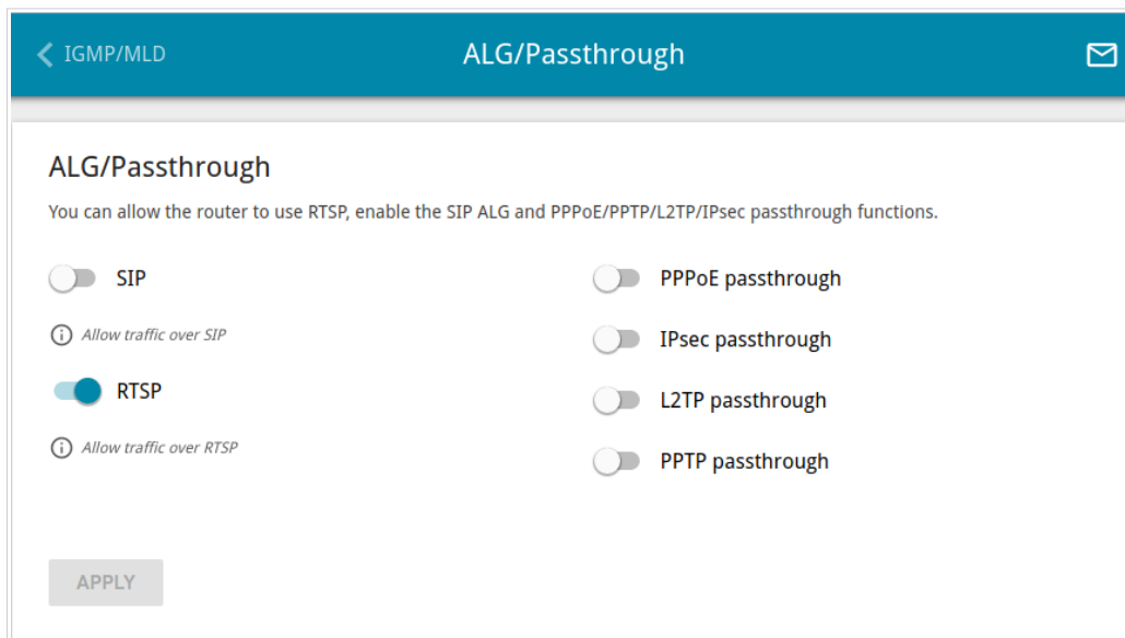
Figure 131. The Advanced / ALG/Passthrough page.
