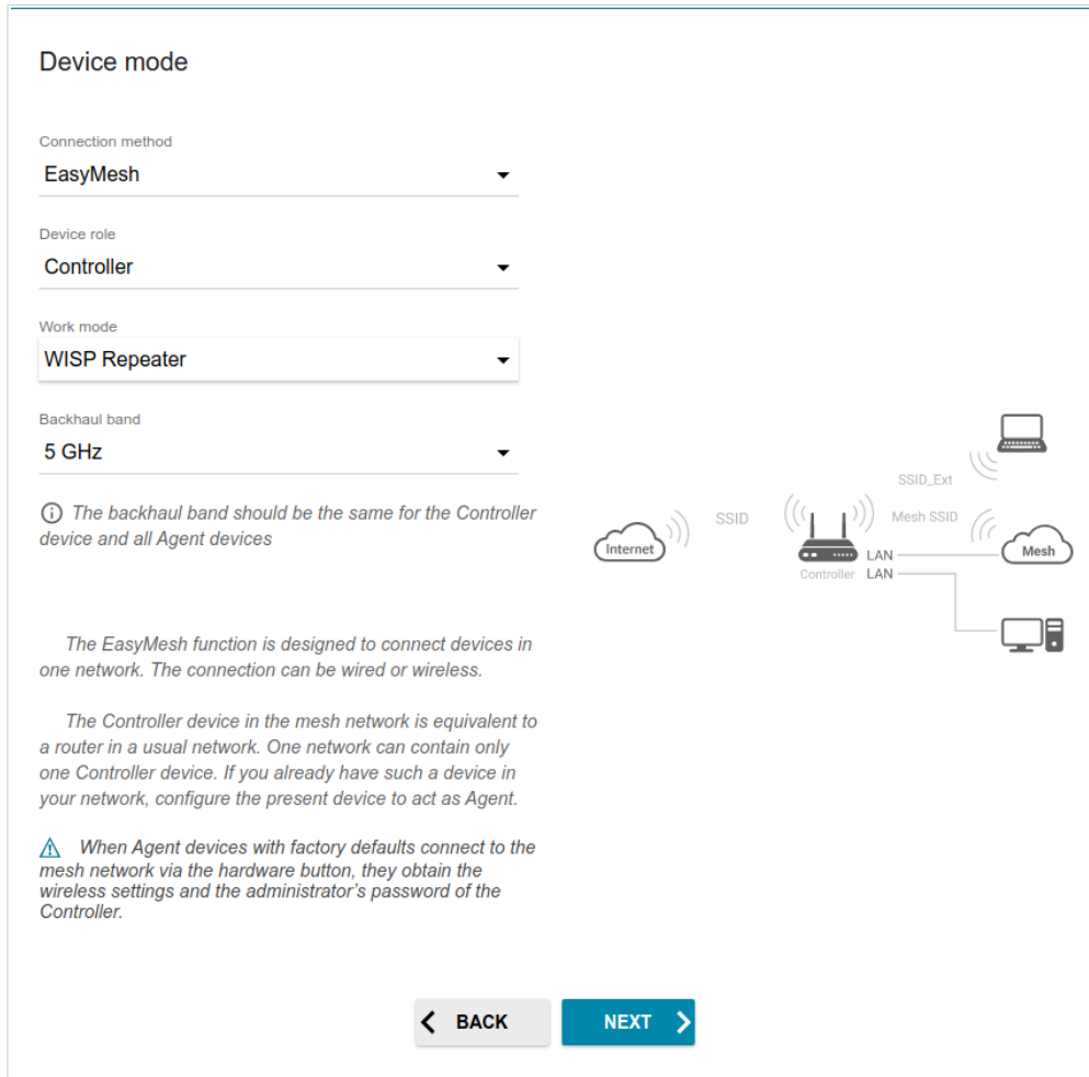
Figure 39. Configuring the EasyMesh function for a main device. The WISP Repeater mode.
