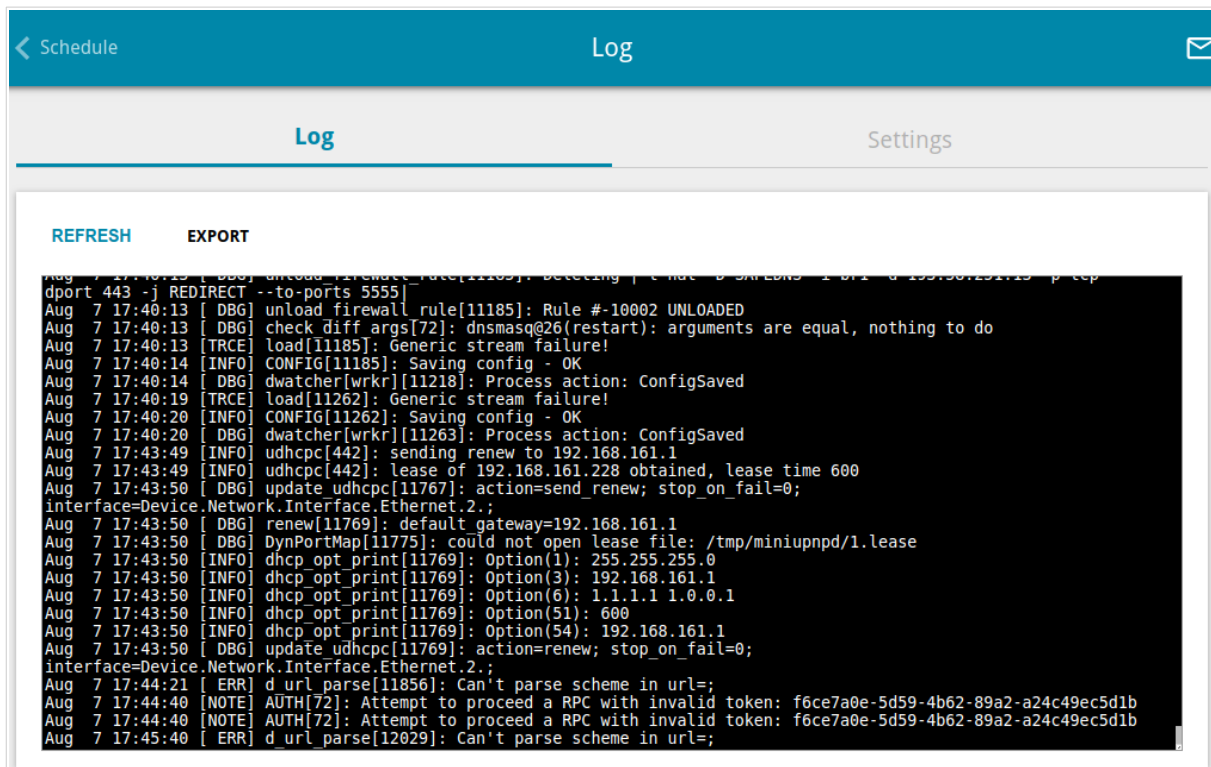
Figure 159. The System / Log page. The Log tab.
