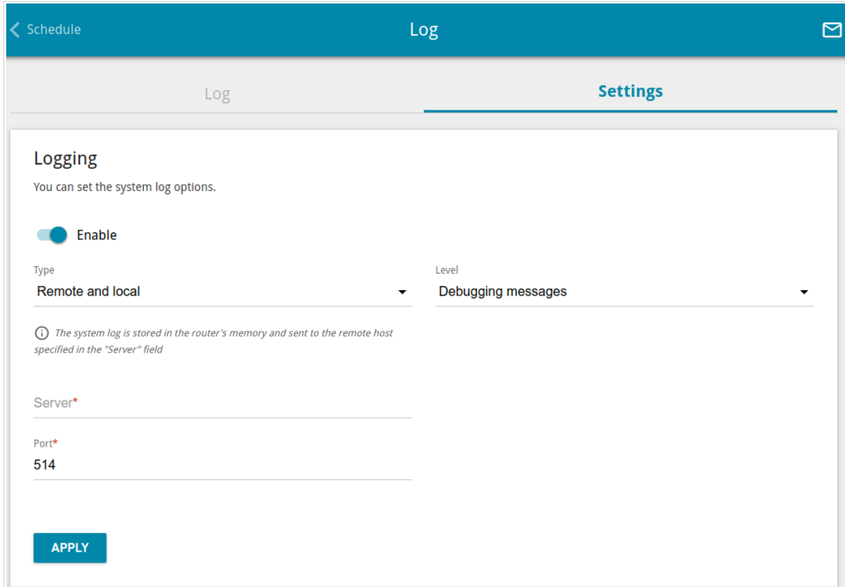
Figure 158. The System / Log page. The Settings tab.
