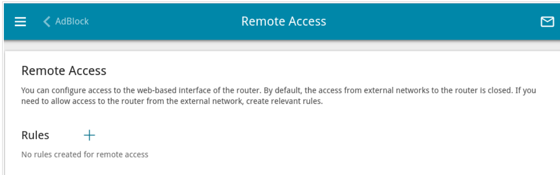
Figure 151. The Advanced / Remote Access page.
