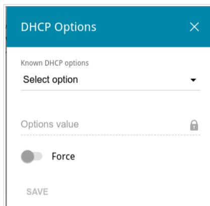
Figure 90. Configuring the local interface. The IPv4 tab. The window for configuring a DHCP option.
