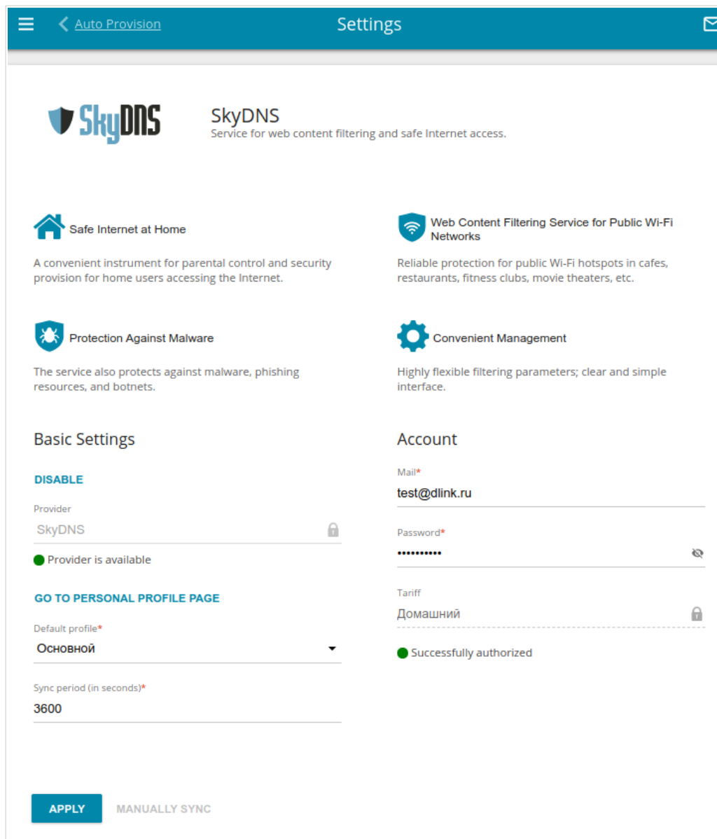
Figure 167. The SkyDNS / Settings page.
