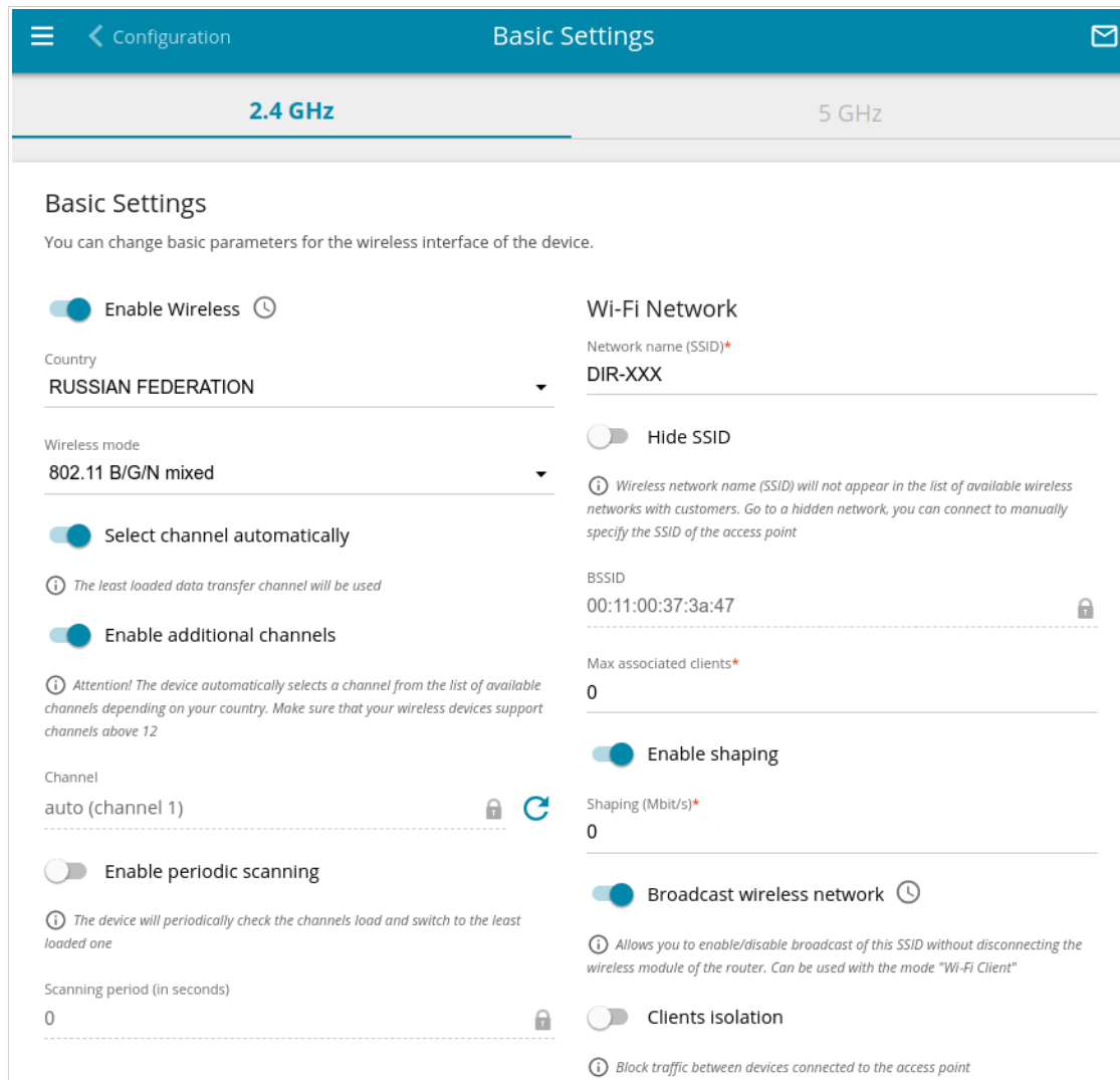
Figure 99. Basic settings of the wireless LAN in the 2.4GHz band.
