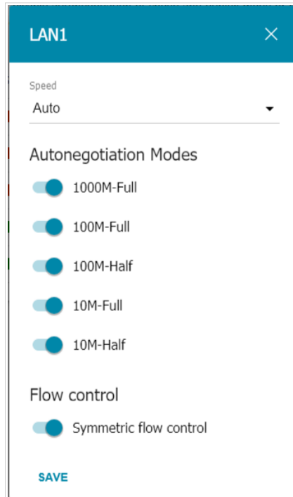
Figure 123. The window for changing the settings of the router's port.
