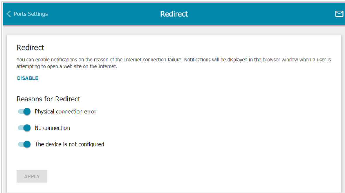
Figure 124. The Advanced / Redirect page.
