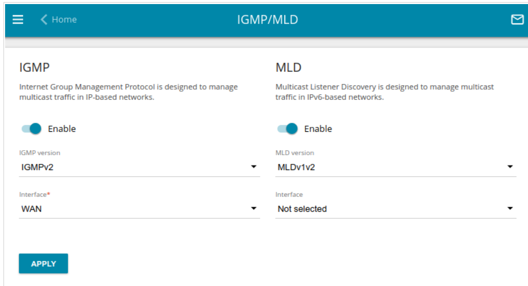
Figure 122. The Advanced / IGMP/MLD page.
