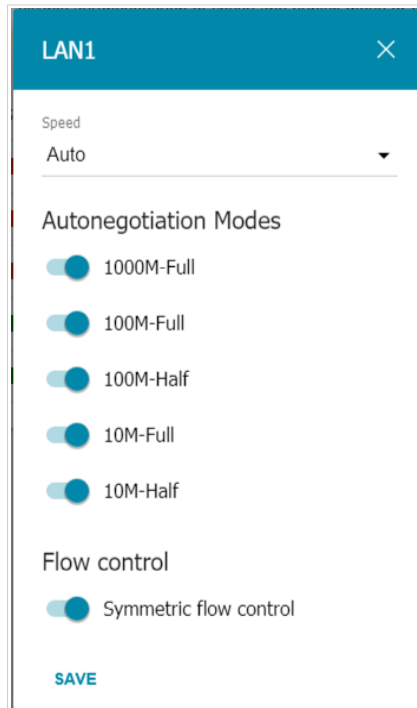
Figure 114. The window for changing the settings of the router's port.
