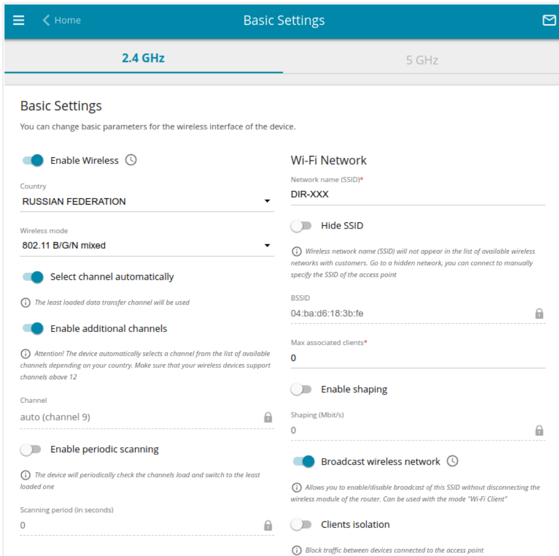
Figure 96. Basic settings of the wireless LAN in the 2.4GHz band.
