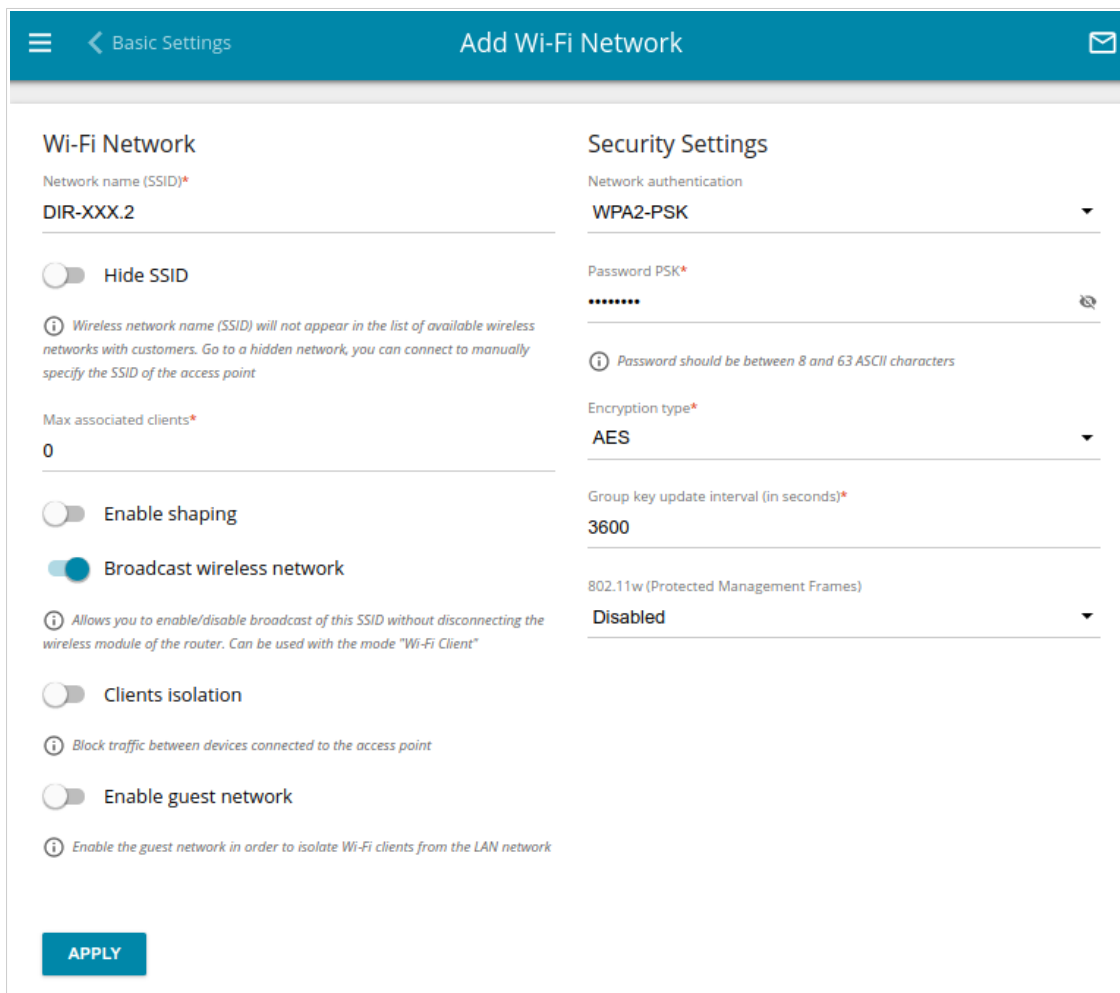
Figure 97. Creating a wireless network.
