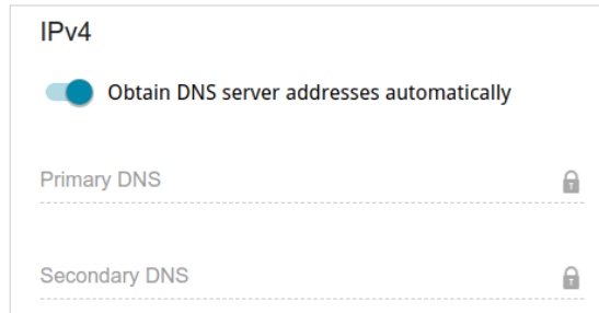
Figure 82. The page for creating a new PPPoE Dual Stack connection. The IPv4 section.
