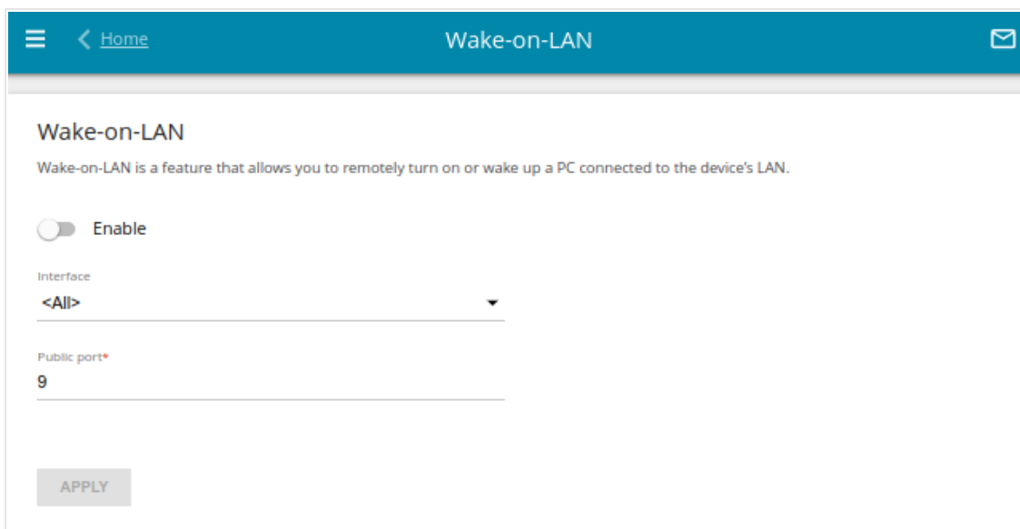
Figure 133. The Advanced / Wake-on-LAN page.
