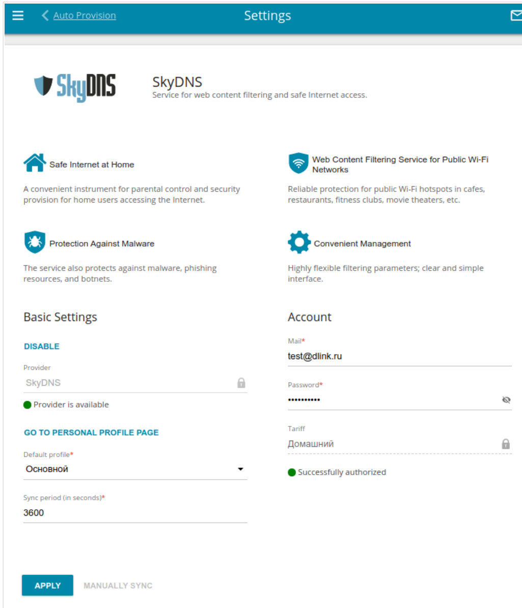
Figure 163. The SkyDNS / Settings page.
