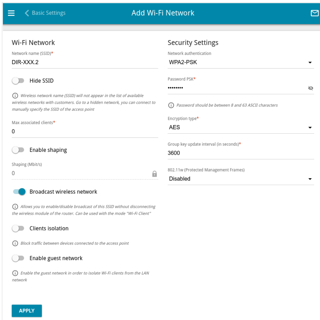
Figure 100. Creating a wireless network.
