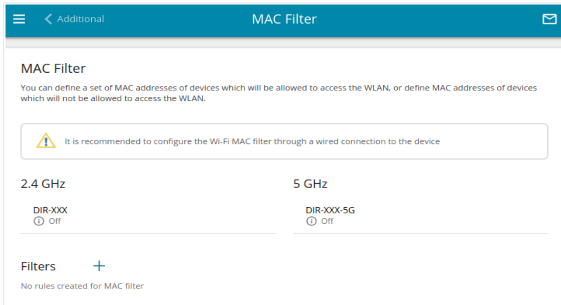
Figure 109. The page for configuring the MAC filter for the wireless network.
