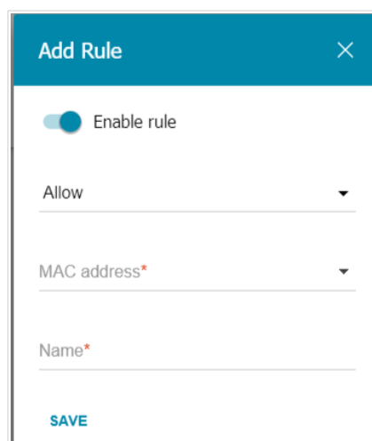
Figure 140. The window for adding a rule for the MAC filter.
