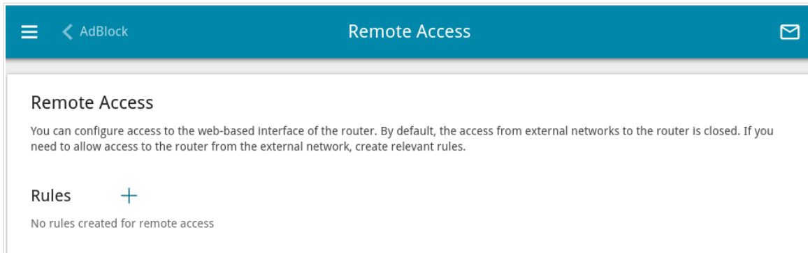
Figure 144. The Firewall / Remote Access page.
