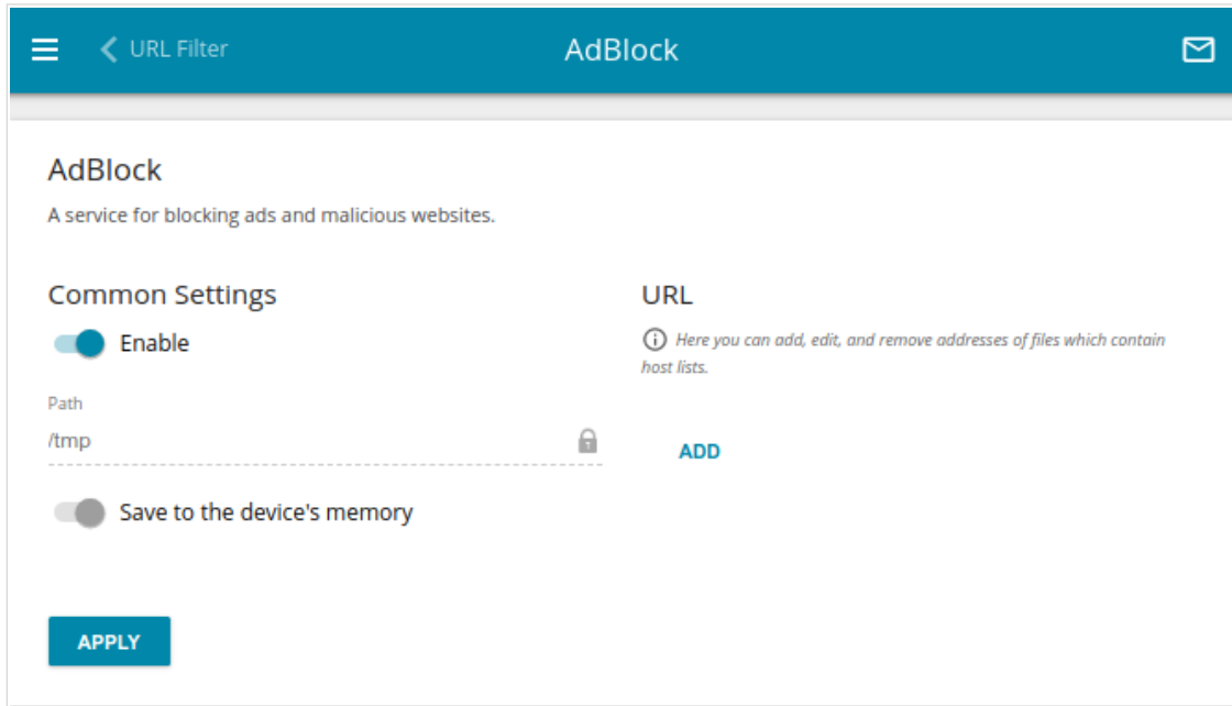
Figure 143. The Firewall / AdBlock page.
