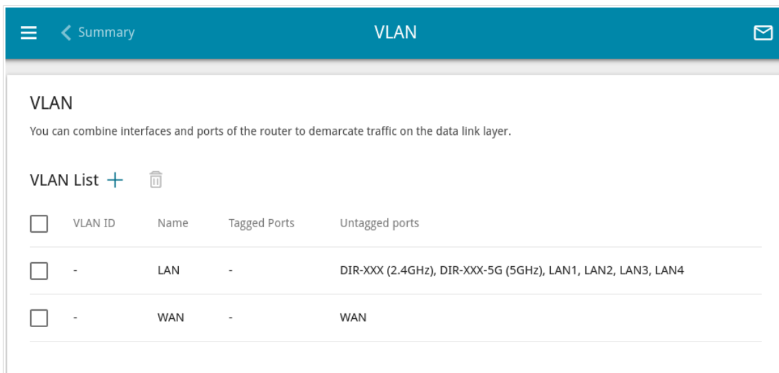
Figure 113. The Advanced / VLAN page.
