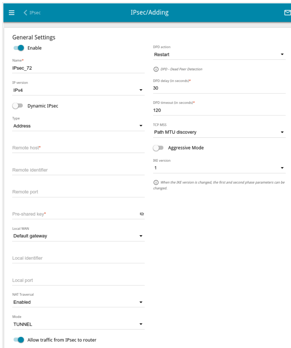
Figure 130. The page for adding an IPsec tunnel. The General Settings section.
