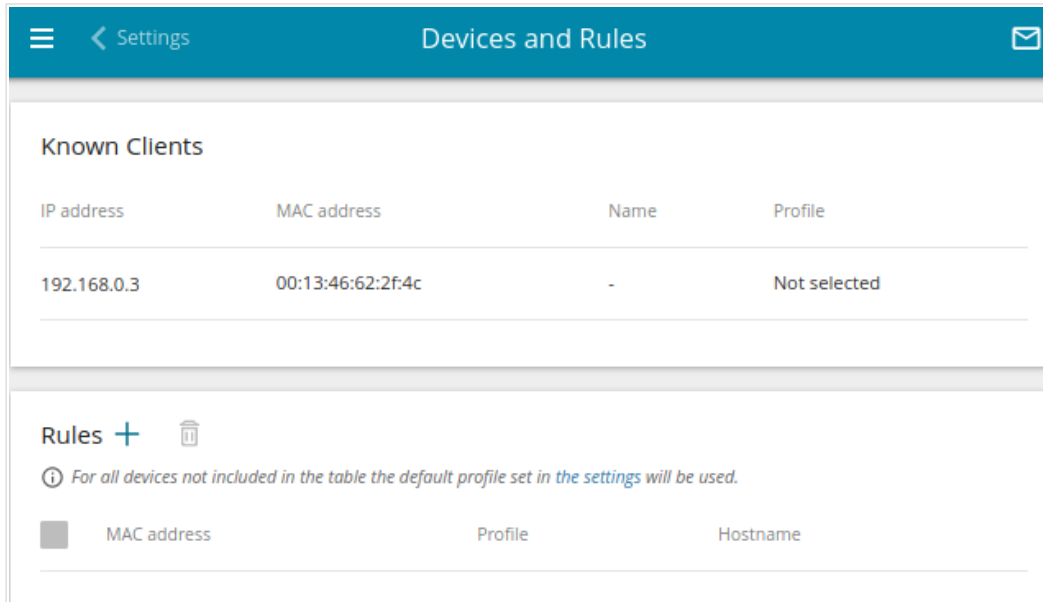
Figure 164. The SkyDNS / Devices and Rules page.
