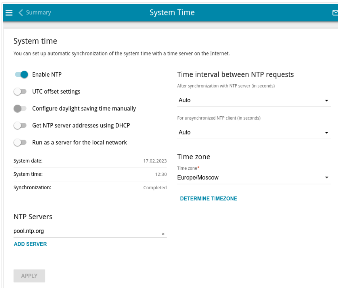
Figure 161. The System / System Time page.
