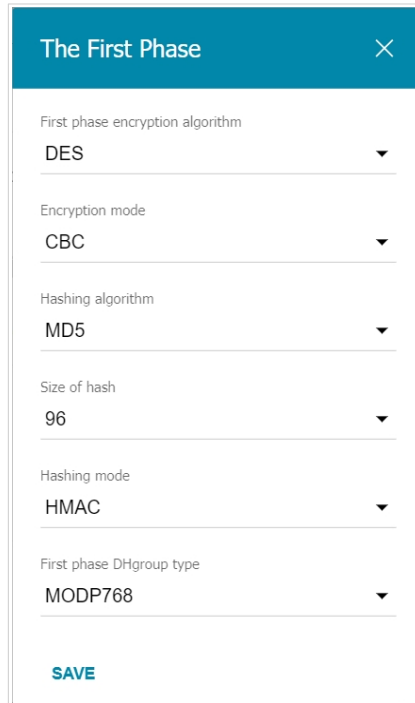
Figure 131. The window for configuring the first phase of the IPsec tunnel. The The First Phase section.
