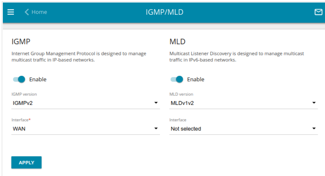
Figure 127. The Advanced / IGMP/MLD page.
