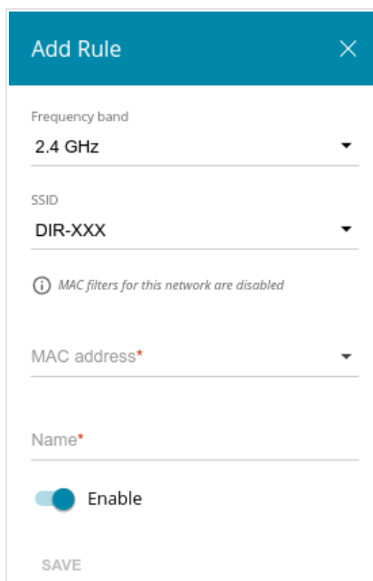
Figure 110. The window for adding a rule for the MAC filter.
