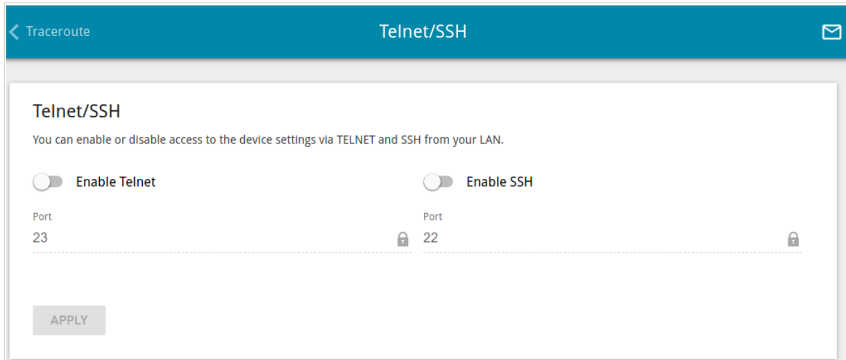
Figure 160. The System / Telnet/SSH page.
