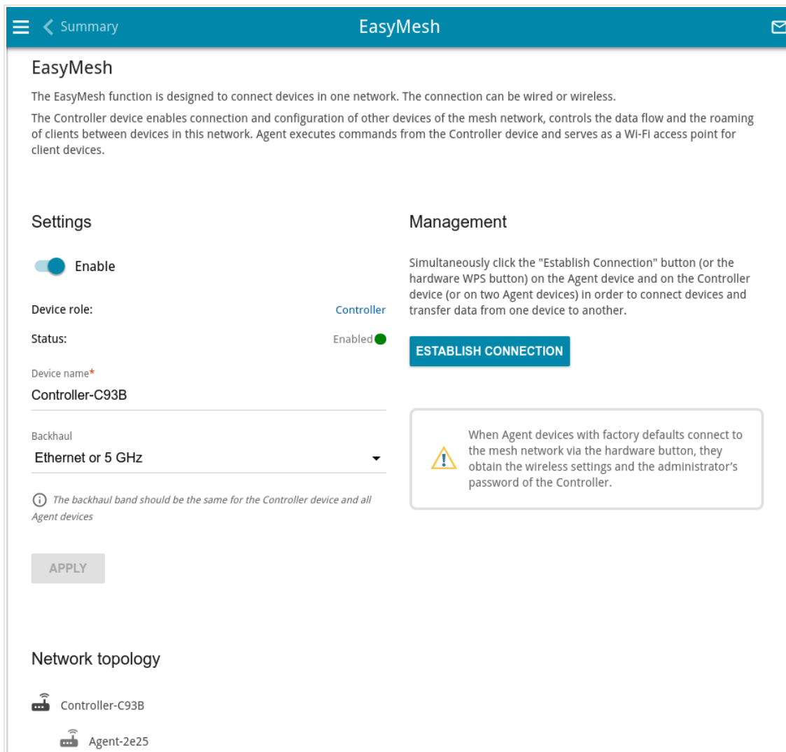
Figure 111. The Wi-Fi / EasyMesh page.
