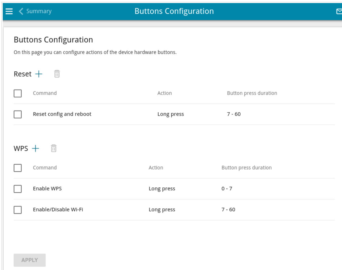
Figure 147. The System / Buttons Configuration page.
