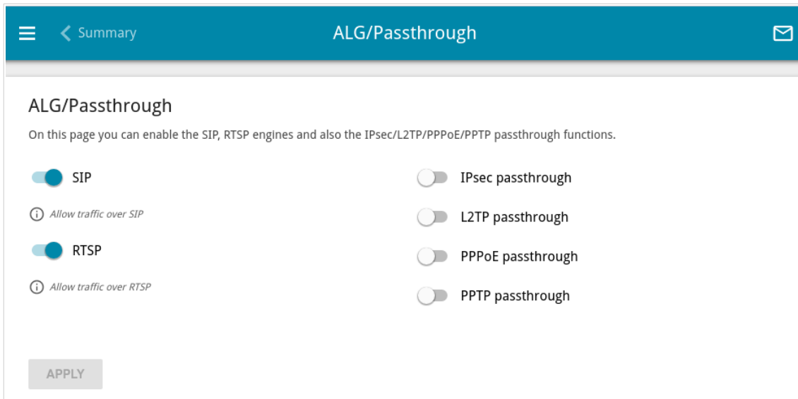
Figure 128. The Advanced / ALG/Passthrough page.
