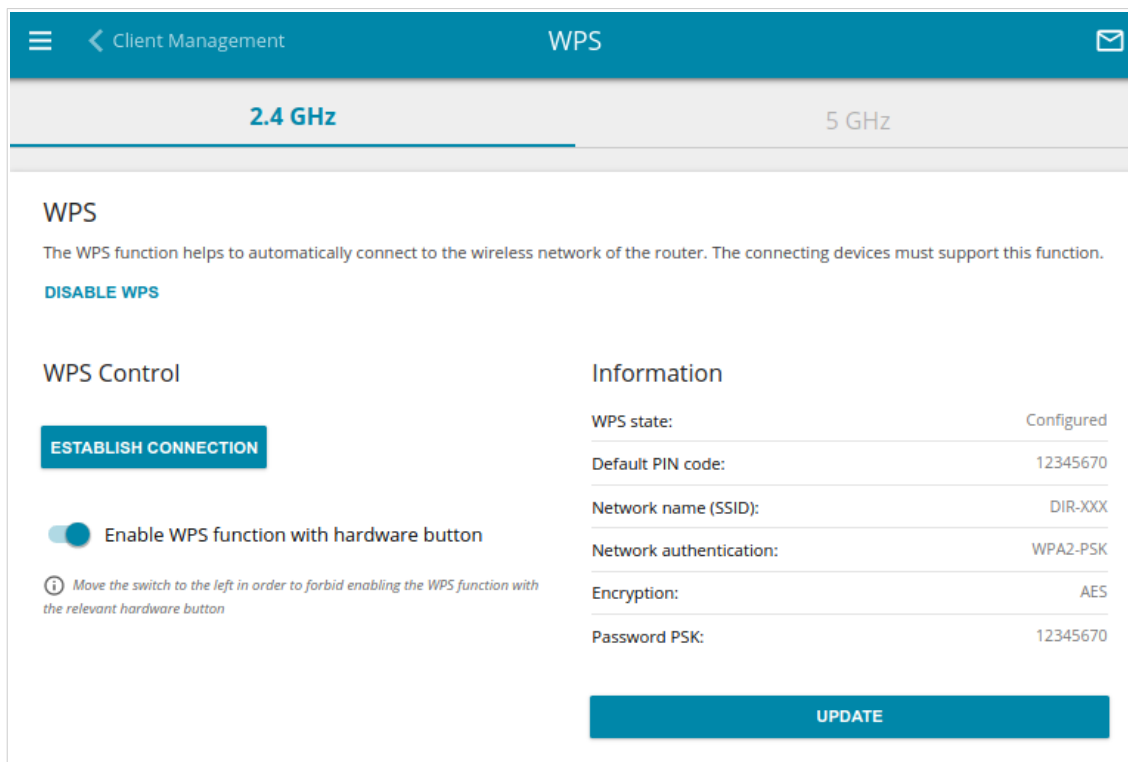
Figure 106. The page for configuring the WPS function.
