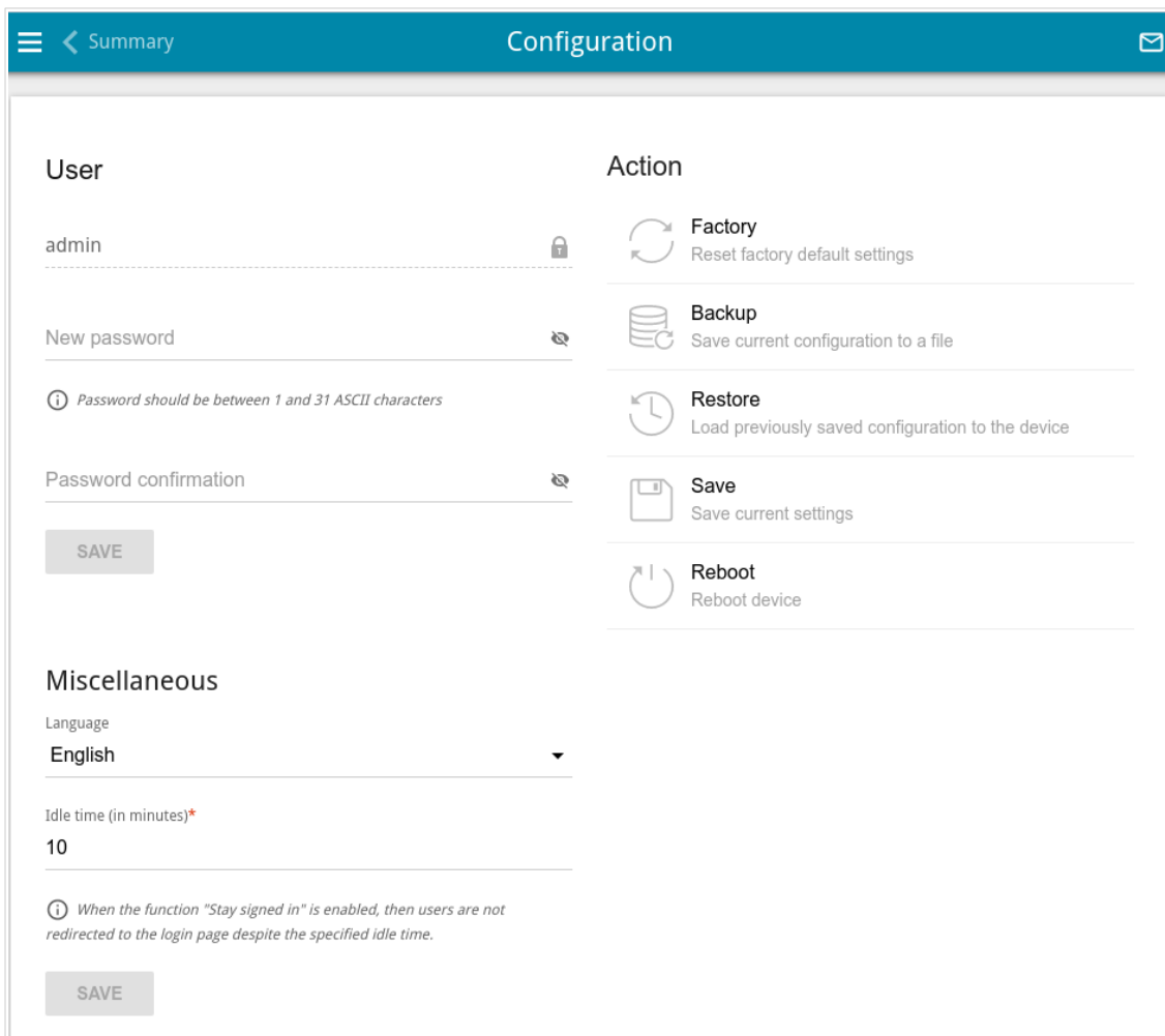
Figure 146. The System / Configuration page.
