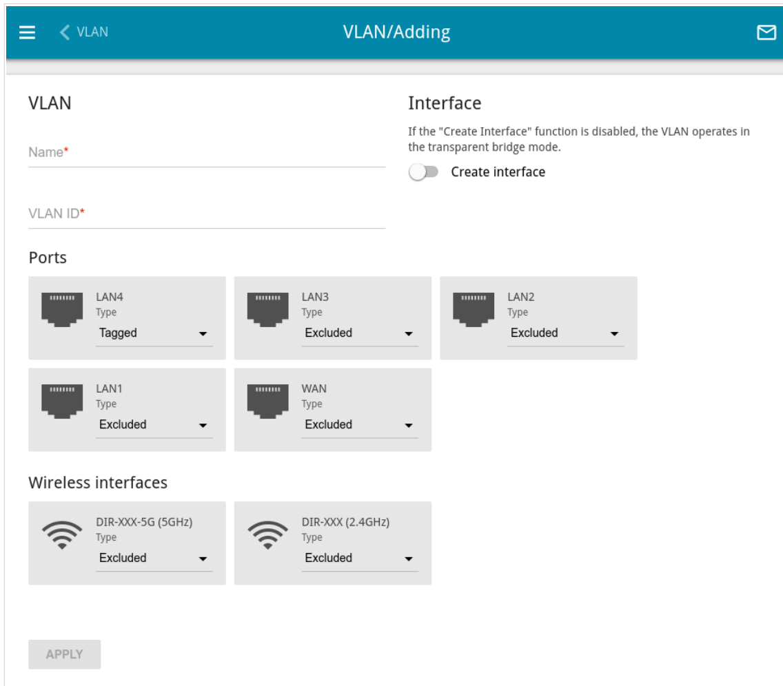
Figure 114. The page for adding a VLAN.
