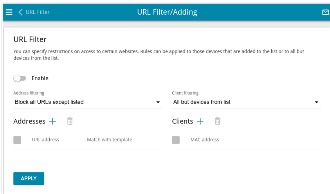
Figure 142. The page for adding a rule for URL filter.
