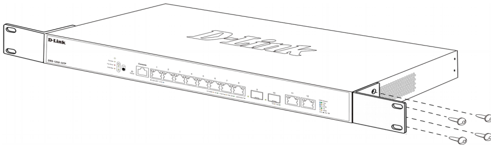
Figure 1 — Attaching rack-mount brackets to the Switch
