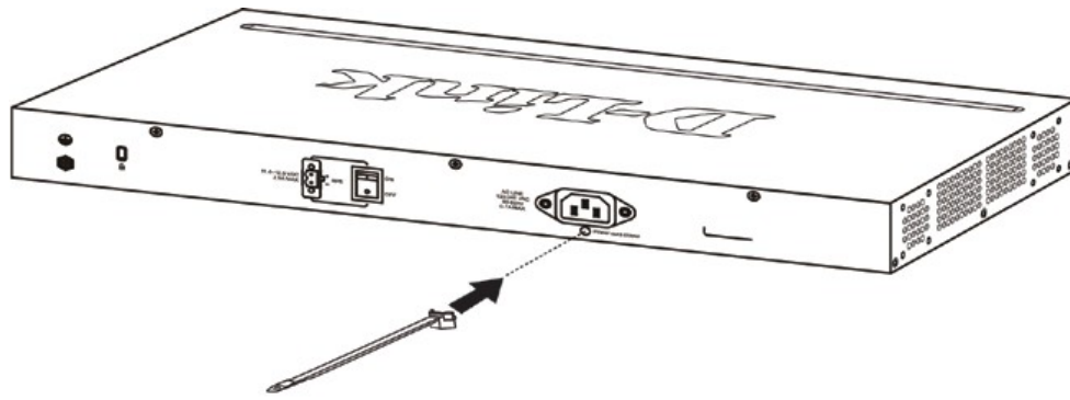
Figure 3 — Insert the tie wrap into the Switch
