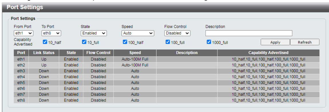
Figure 4.17 - System > Port Configuration > Port Settings
