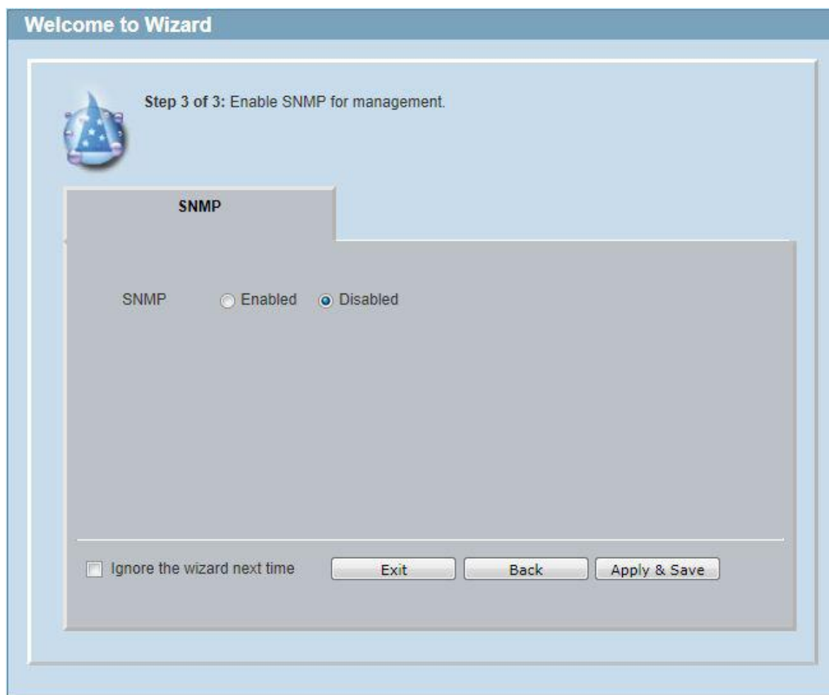
Figure 4-6 SNMP window
