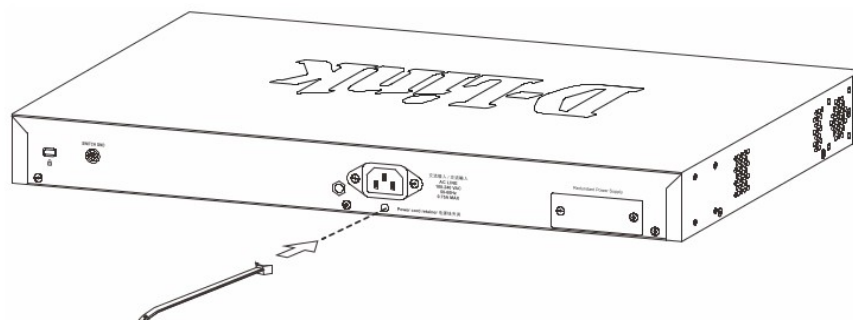
Figure 5 — Insert Tie Wrap into the Switch
