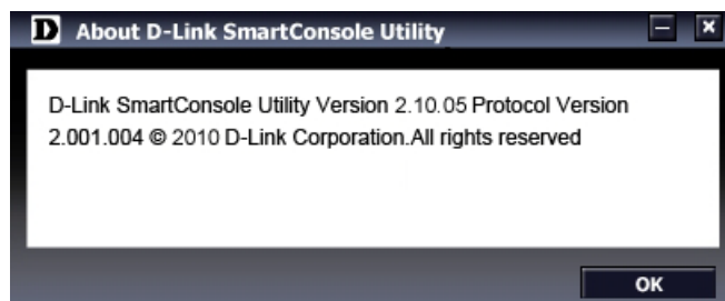
Figure 4.6 – SmartConsole Help
