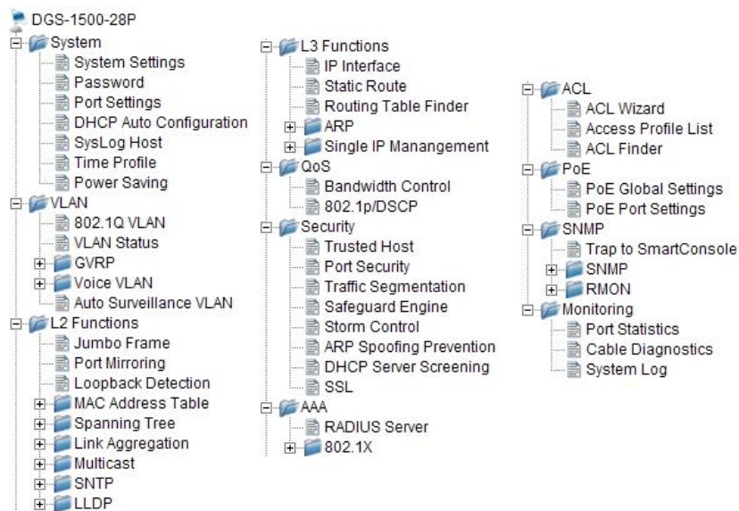
Figure 5.16 –Function Tree
