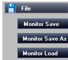
Figure 4.5 – SmartConsole File
