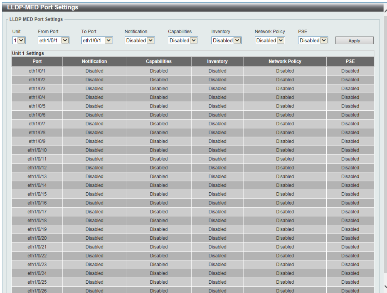
Figure 5-78 LLDP-MED Port Settings Window
