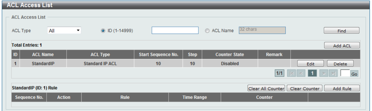
Figure 8-21 Standard IP ACL (Selected) Window
