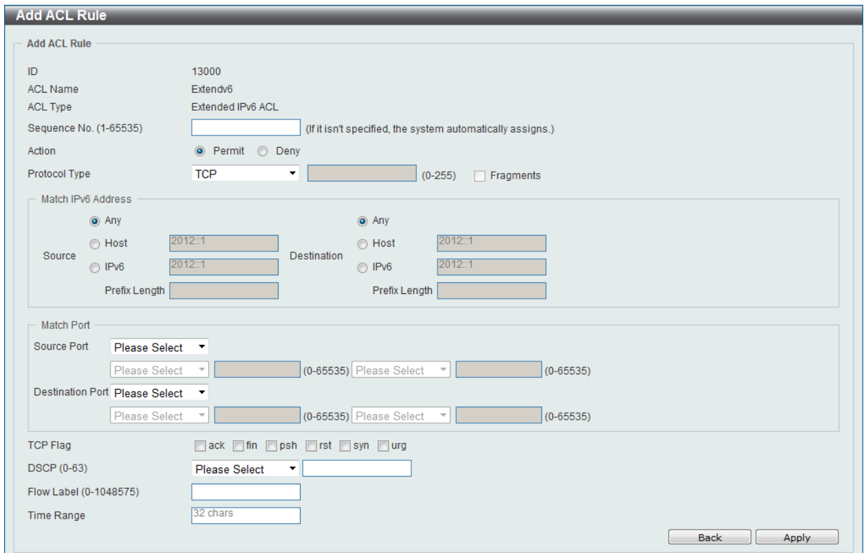
Figure 8-44 Extended IPv6 ACL (Add Rule) Window
