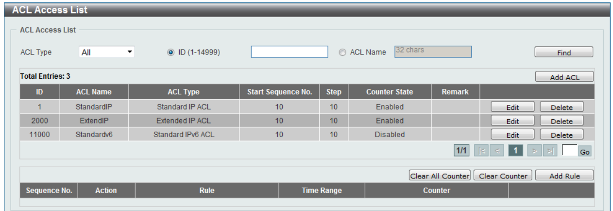
Figure 8-36 Standard IPv6 ACL (Main) Window
