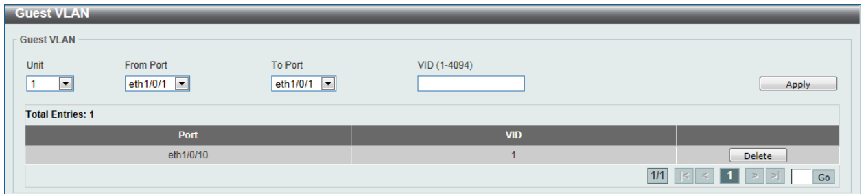
Figure 9-75 Guest VLAN Window
