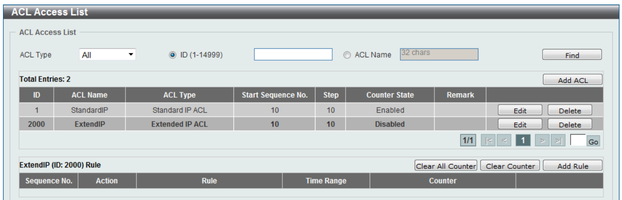
Figure 8-27 Extended IP ACL (Selected) Window
