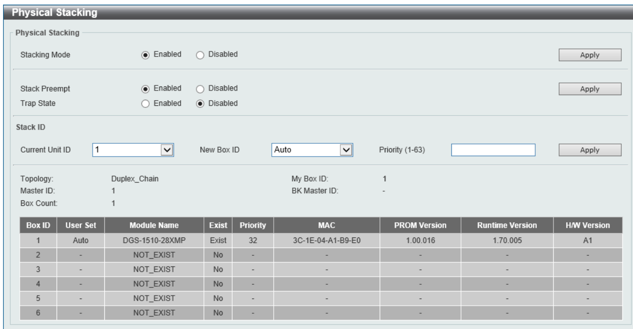
Figure 4-75 Physical Stacking Window
