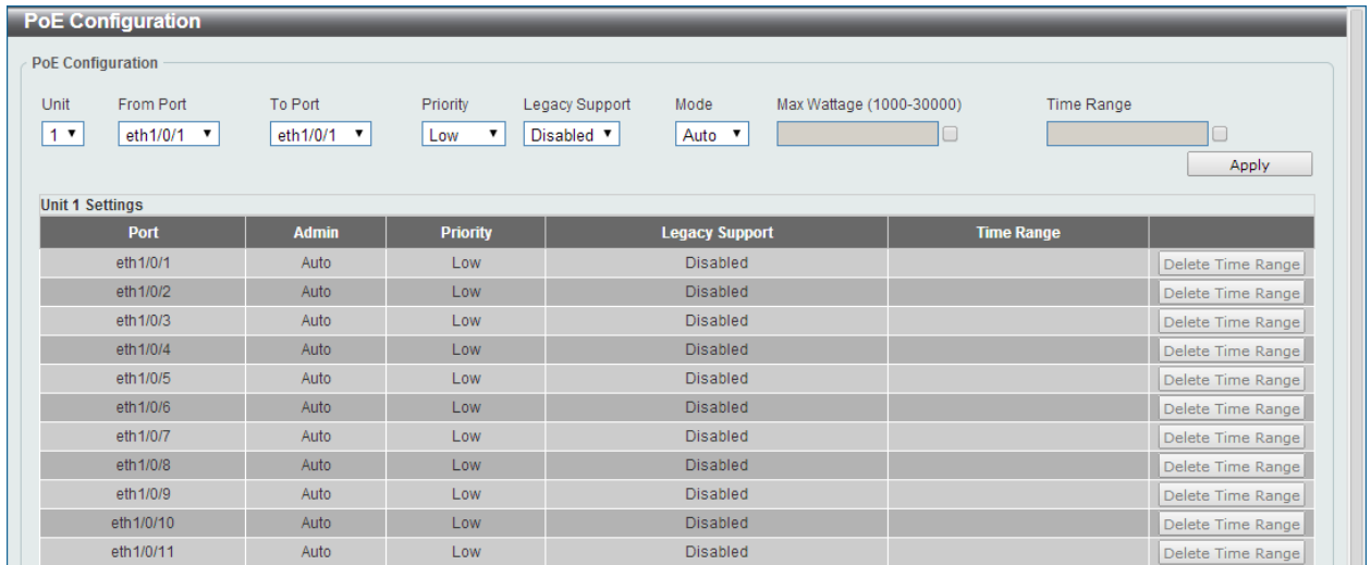
Figure 3-14 PoE Configuration Window
