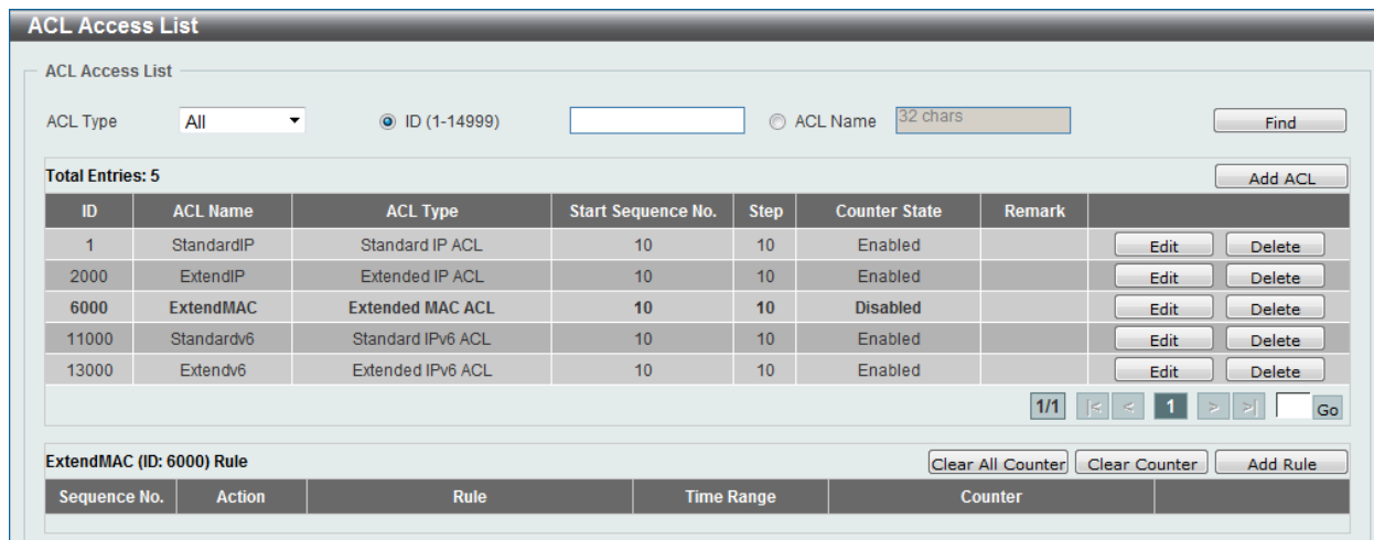
Figure 8-53 Extended MAC ACL (Selected) Window
