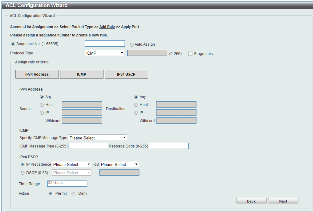
Figure 8-8 ACL Configuration Wizard (Add Rule for IPv4 ACL) ICMP Window
