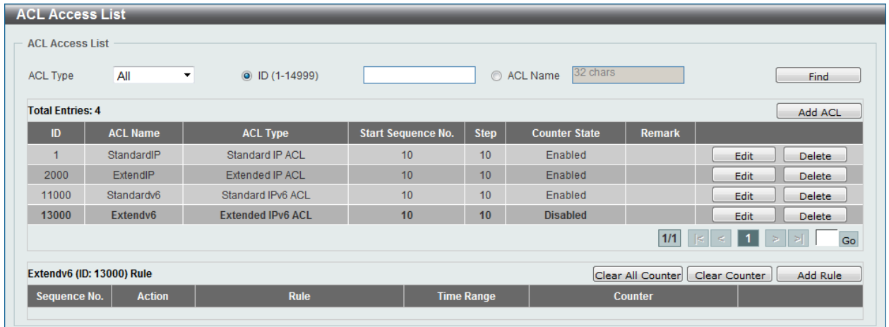
Figure 8-43 Extended IPv6 ACL (Selected) Window
