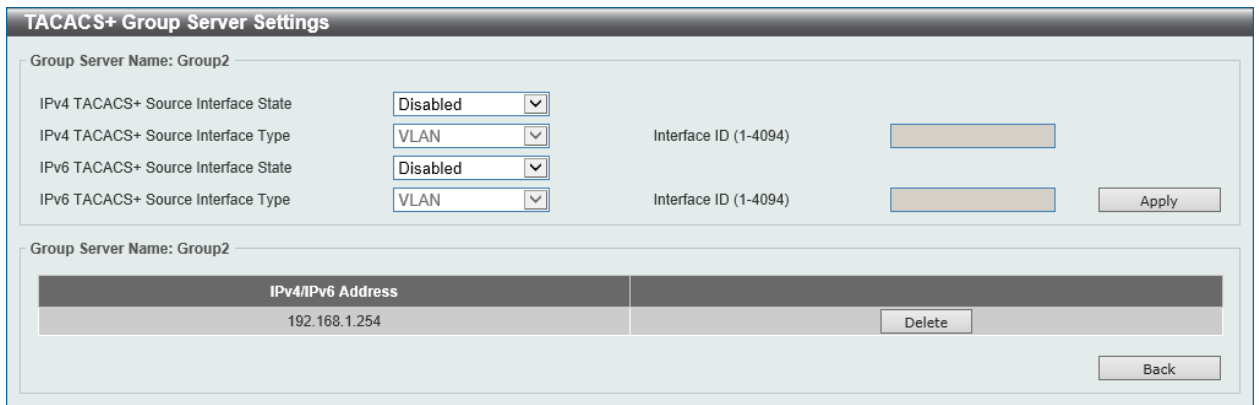
Figure 9-36 TACACS+ Group Server Settings - Detail Window
