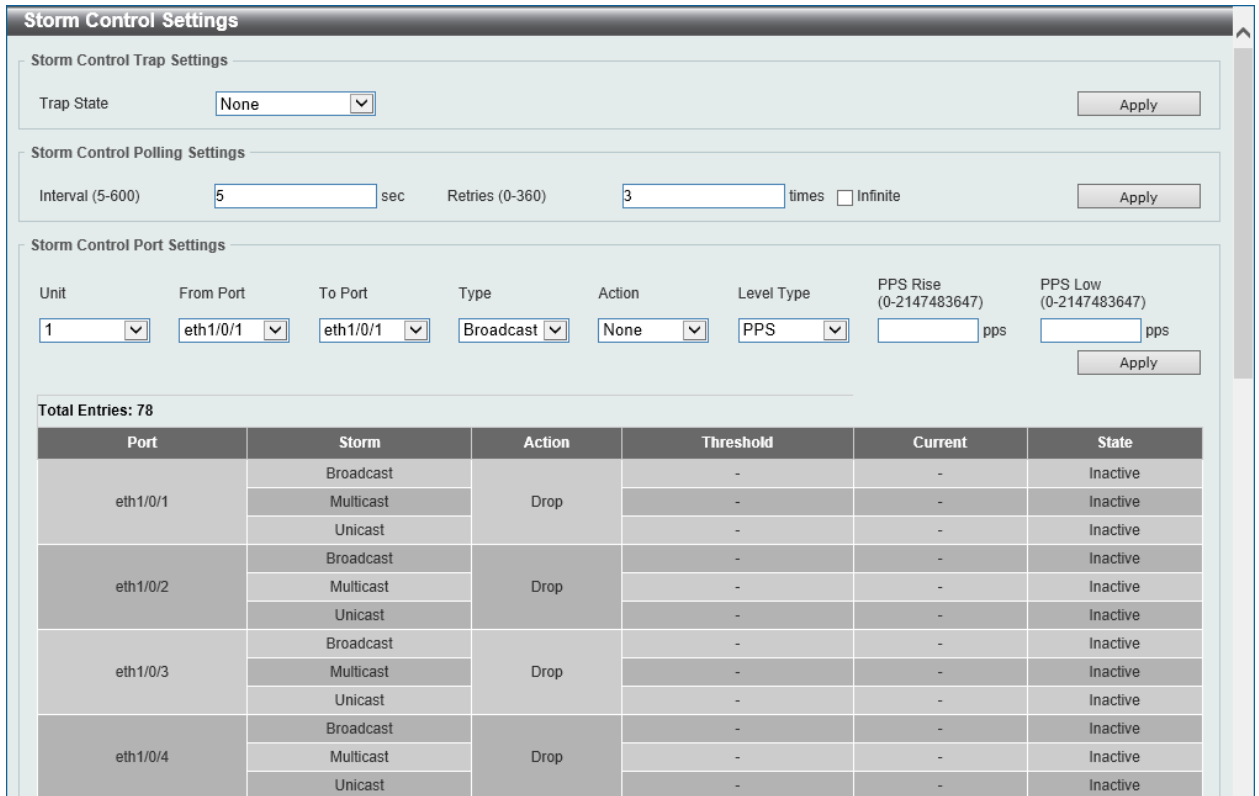
Figure 9-85 Storm Control Settings Window
