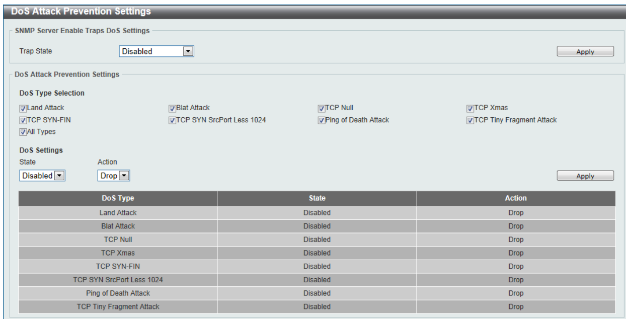
Figure 9-88 DoS Attack Prevention Settings Window
