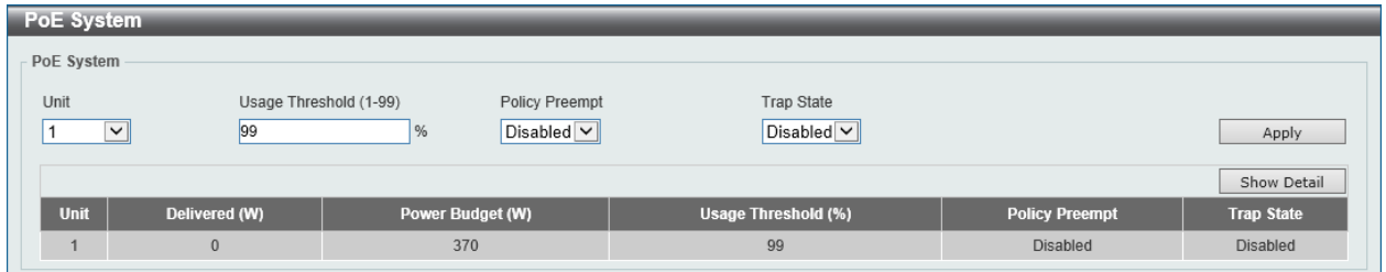
Figure 3-11 PoE System Window
