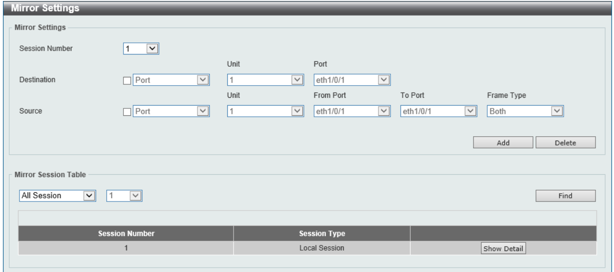
Figure 11-8 Mirror Settings Window
