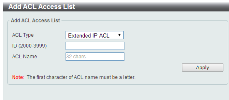
Figure 8-25 Extended IP ACL (Add Profile) Window
