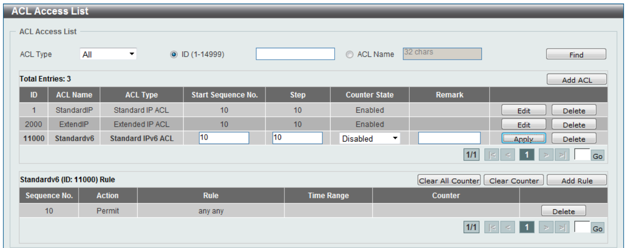
Figure 8-39 Standard IPv6 ACL (Edit ACL) Window
