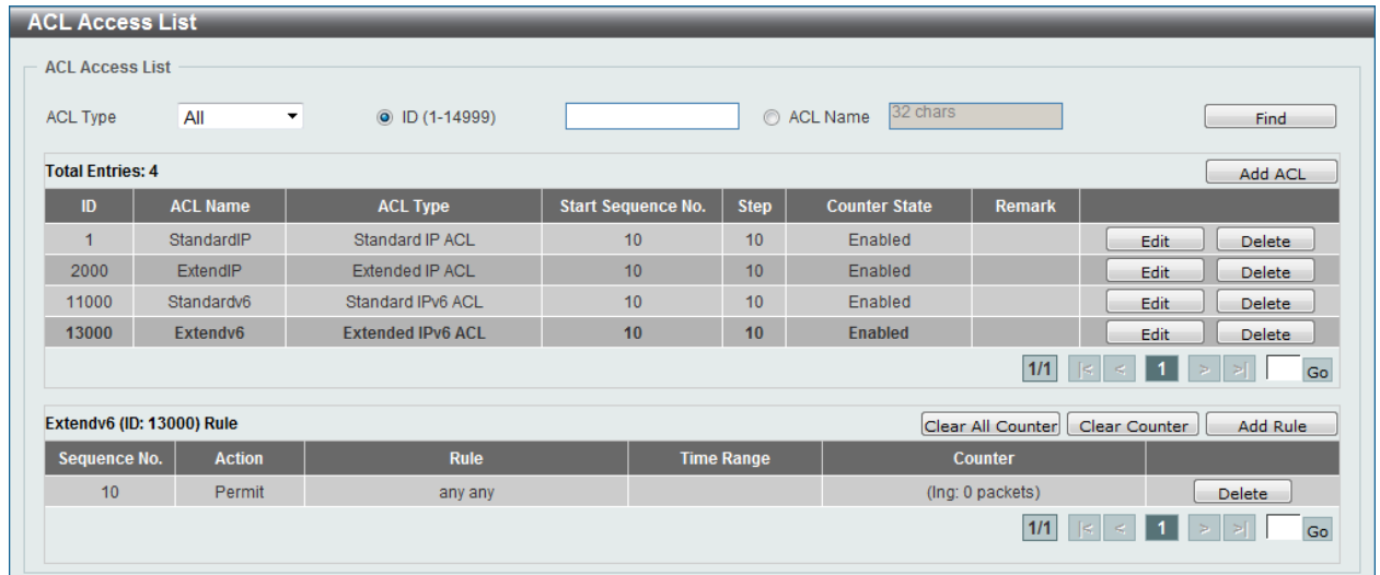
Figure 8-50 Extended IPv6 ACL (Rule Display) Window
