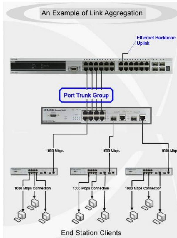
Figure 5-56 Example of Port Trunk Group
