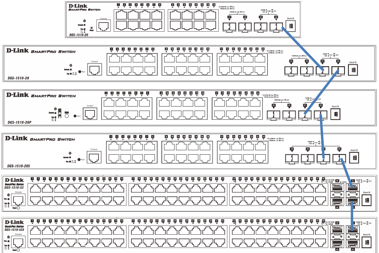
Figure 4-73 Switches stacked in a Duplex Chain
