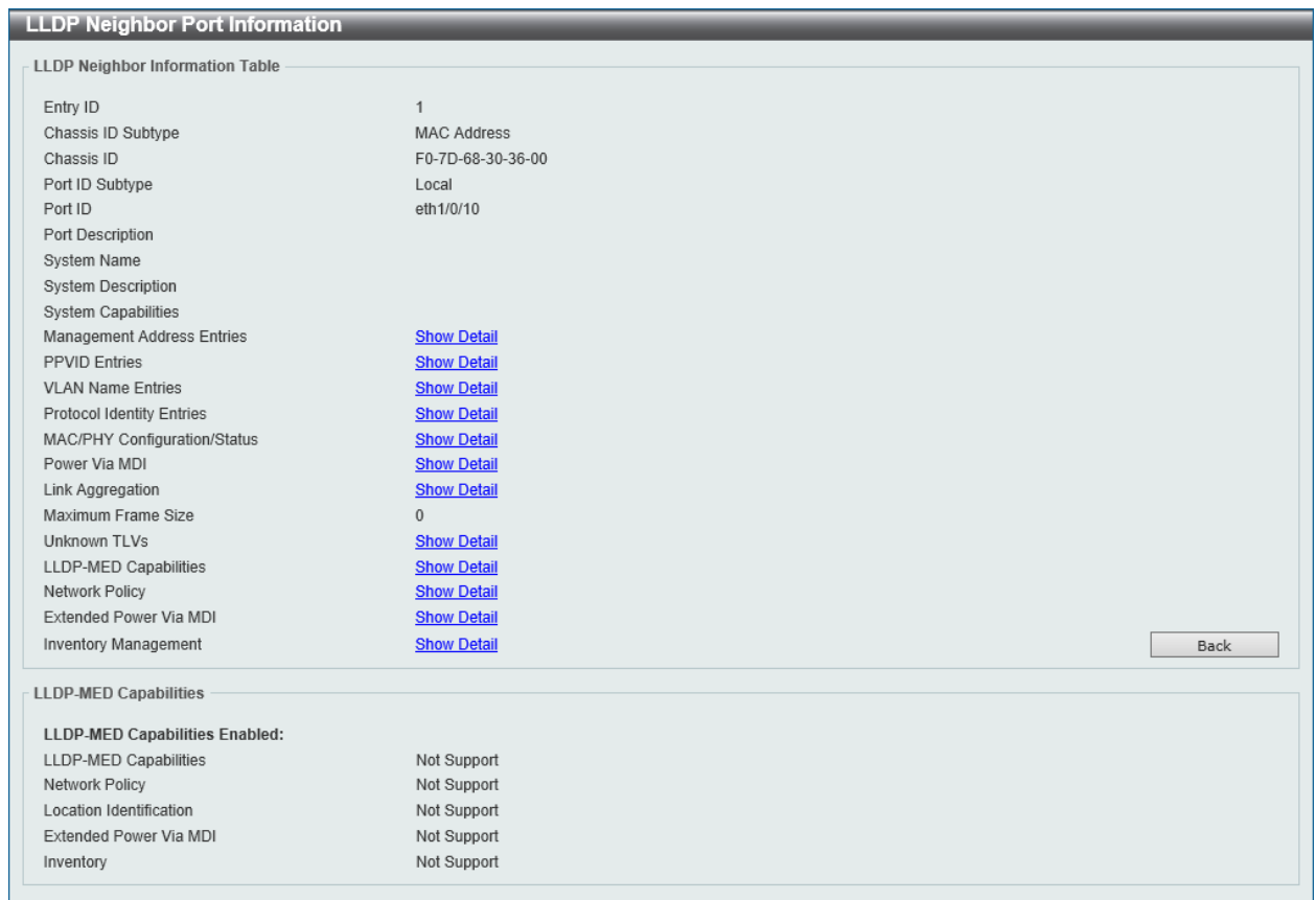
Figure 5-85 LLDP Neighbor Port Information - Show Detail Window
