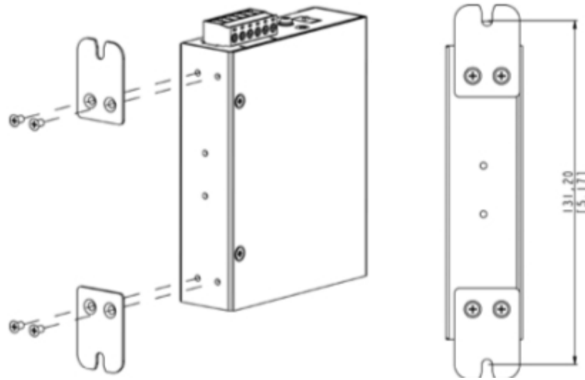
5-Port Model
