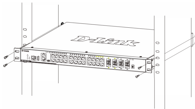
Figure 3 — Installing the Switch in a rack
