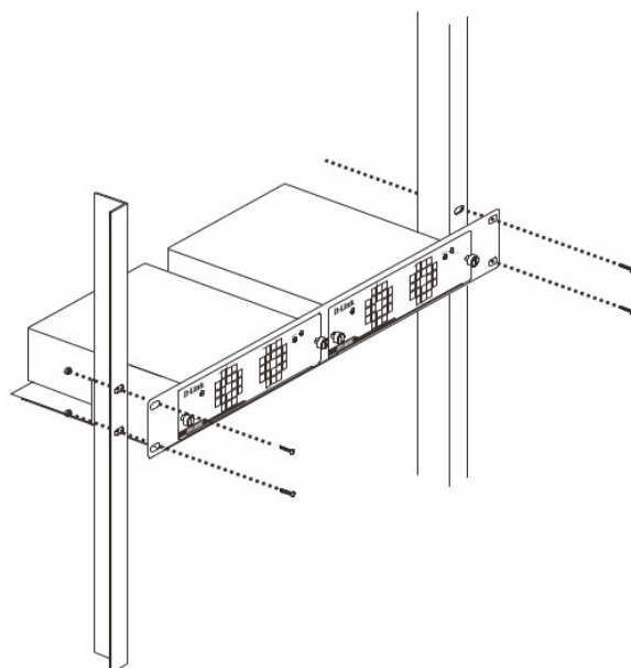
Figure 7 — Install the DPS-800 in an equipment rack
