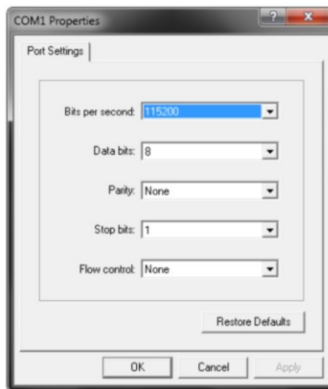
Figure 8 — COM Port Configuration
