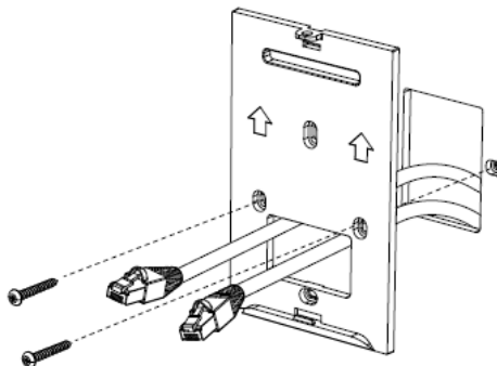
Figure 4: Attaching the Mounting Plate
