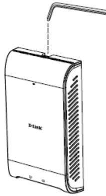
Figure 6: Mounting the Device
