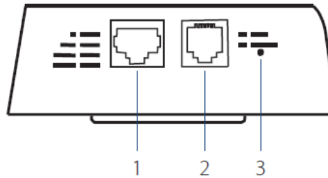
Figure 2: Bottom Connectors
