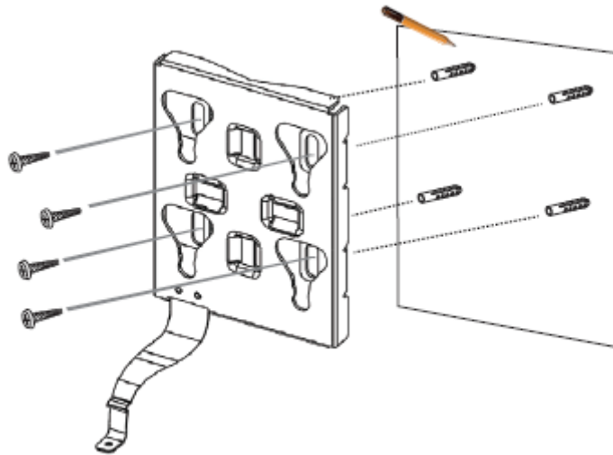
Figure 7: Attaching the Mounting Plate
